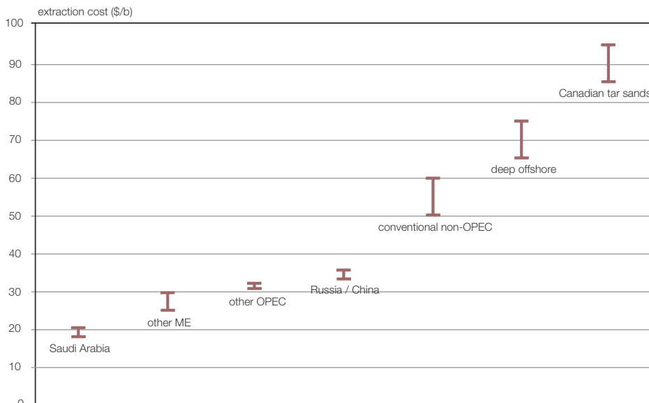
Fig 2.4 For a range of oil sources, comparison of extraction costs. (ME: Middle East countries) (Source: Peak Oil Consulting)
