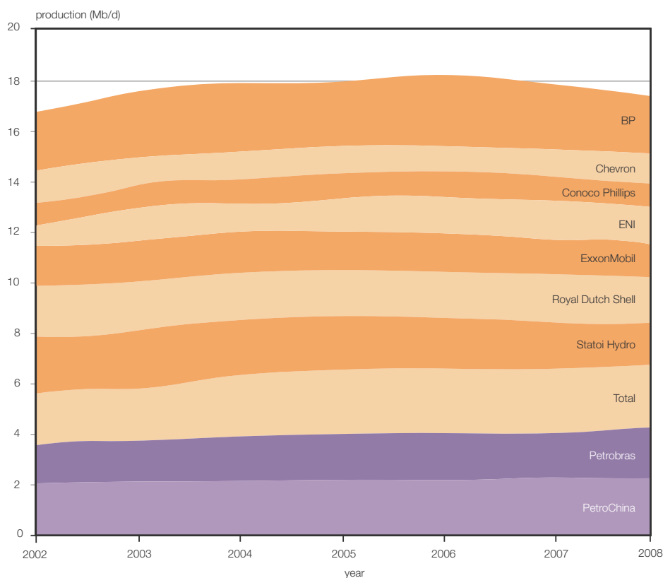
Fig 2.5 Aggregated production for the world's ten largest quoted oil companies. (Source: Peak Oil Consulting)
