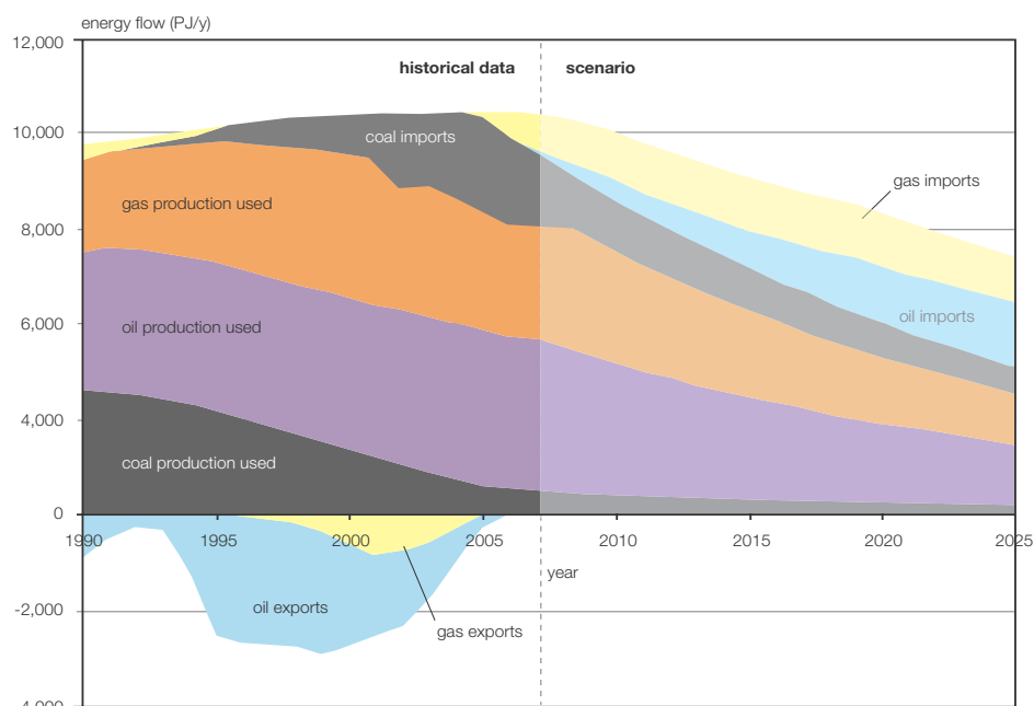
Fig D.7 Extraction, use and trade of coal, oil and gas for the historical period to 2007 and projected to 2025 according to the proactive investment scenario together with decline of North Sea oil and gas production at 5 percent per year.
