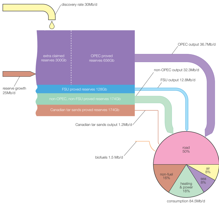
Fig 2.6 Schematic of the size of oil reserves, supply and demand in today's market. Non-fuel consumption includes chemicals, solvents, lubricants and asphalt. (Source: Peak Oil Consulting)
