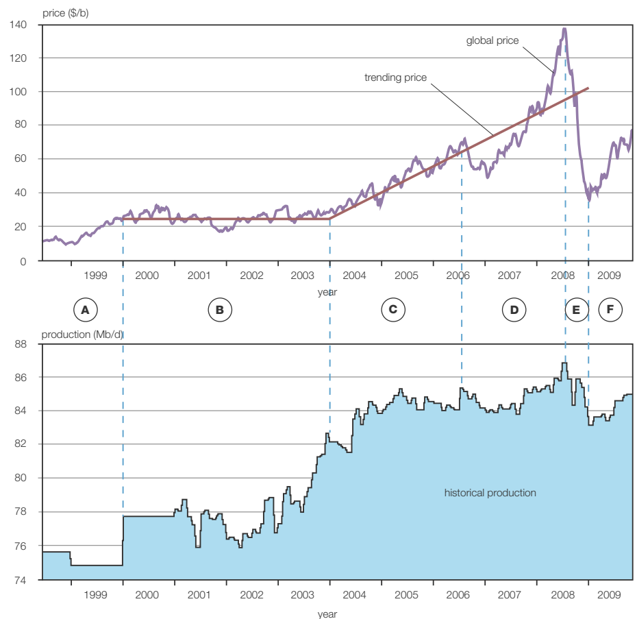
Fig 3.1 Global price and historical production for crude oil in the last decade showing the basic forces acting on the industry since 2000. (Source: EIA production and prices)
