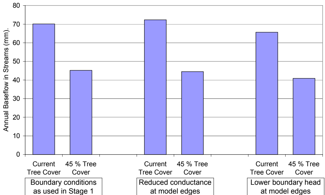
■ Figure 4-7 Stream baseflow output by MODFLOW for two land use conditions and three different configurations of the GHB boundaries at the edge of the model.
