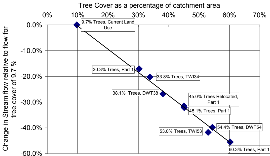
■ Figure 5-1 Gardiner Creek: change in modelled stream flow versus tree cover. The line shown is the linear regression line that passes through the point representing current conditions (i.e. stream flow = 108 mm/y). The data point labels are described in the text.
