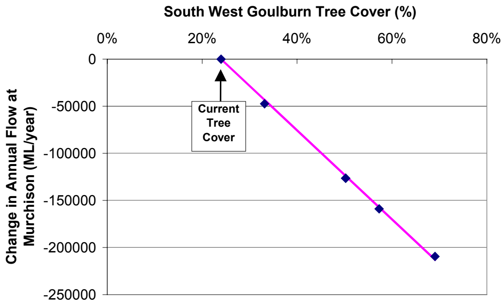
■ Figure 5-6 Change in modelled annual flow at Murchison vs tree cover in the South West Goulburn.
