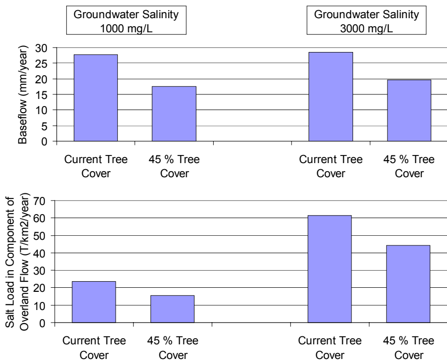
■ Figure 4-10 Gardiner Creek: Comparison of the effects of groundwater salinity on different components of salt and water balance.
