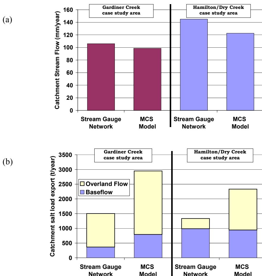
■ Figure 3-1 Average annual runoff (a) and salt load export (b) from the case study areas (as presented in Part 1 of the project).
