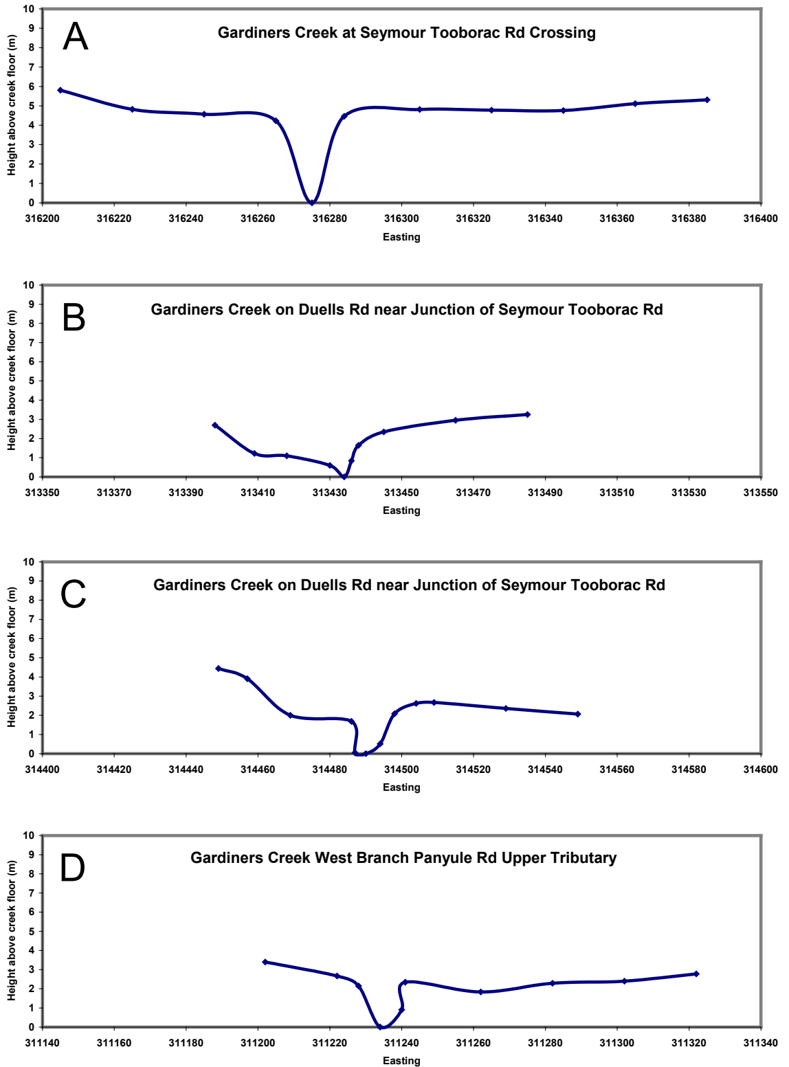
■ Figure B.3 Surveyed cross sections Gardiner Creek
