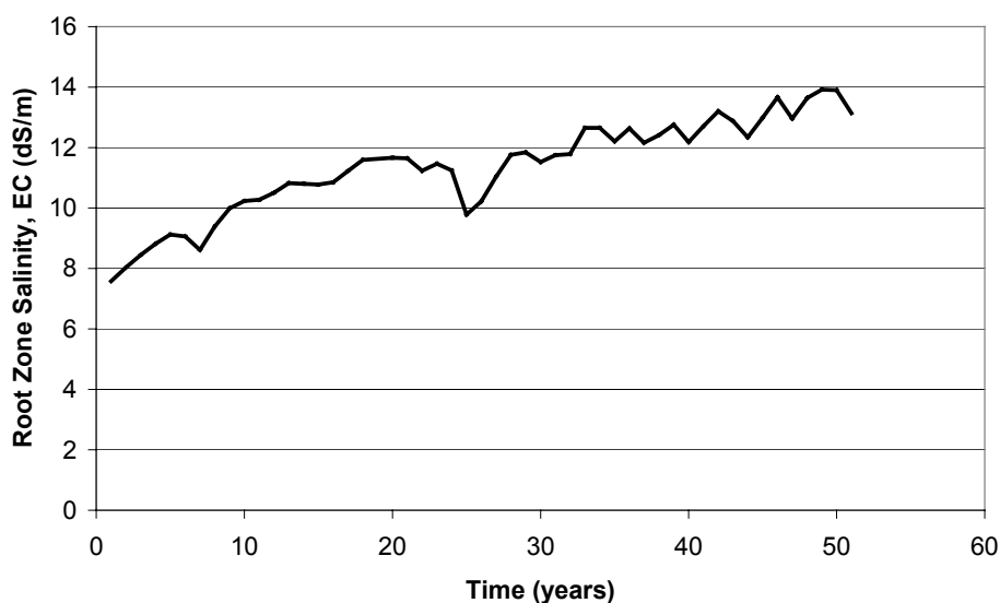
■ Figure 4-12 Gardiner Creek: Time series of root zone salinity for a land use of trees with an underlying groundwater potential equivalent to a watertable depth of 0.5 m.
