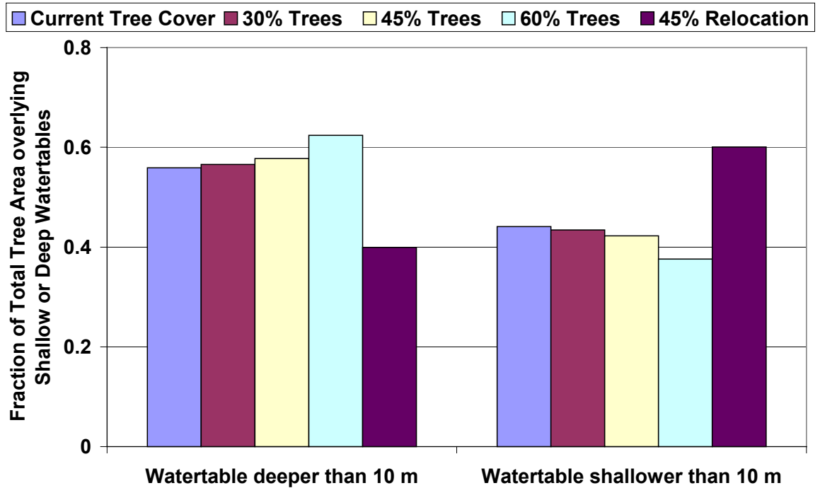
■ Figure 3-6 Hamilton/Dry: depth of watertable underlying trees for different tree cover scenarios (scenarios taken from Part 1 of the project).
