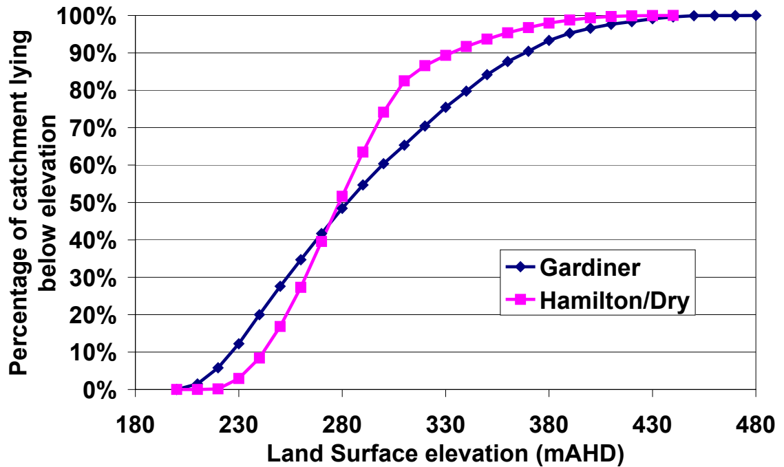
■ Figure 3-7 The distribution of land surface elevations in the case study areas.
