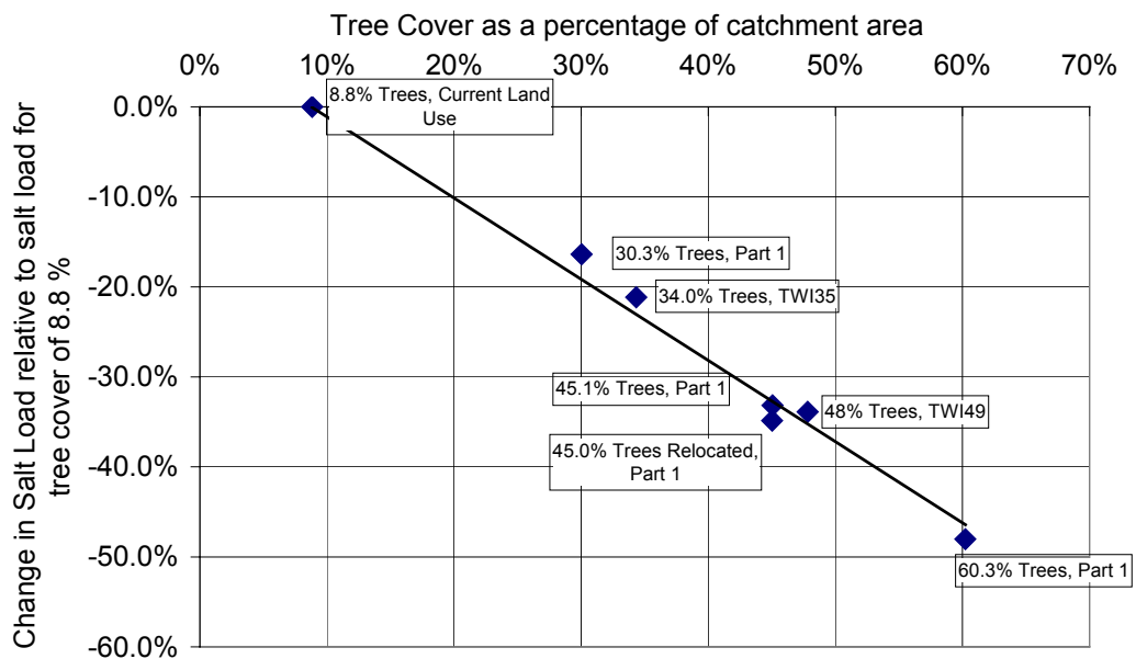
■ Figure 5-4. Hamilton/Dry case study area: change in modelled salt load export versus tree cover. The line shown is the linear regression line passing through the point representing current conditions (i.e. tree cover = 8.8 %, salt load = 51 T/km 2 /year).
