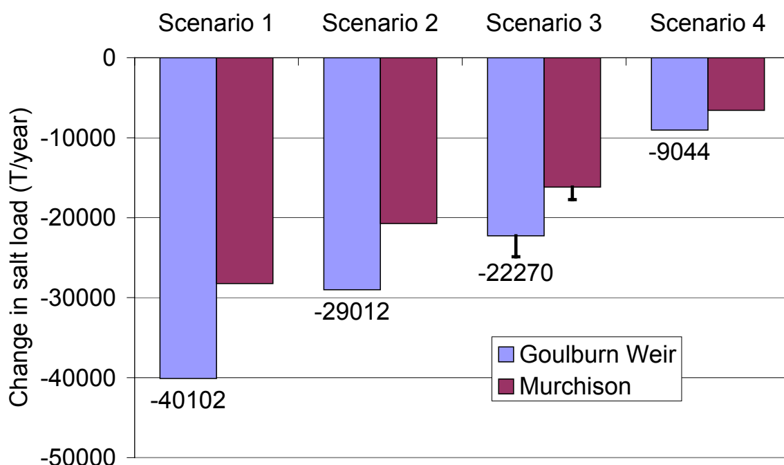
■ Figure 5-5 Change in salt load carried by the Goulburn River as modelled by REALM for the four scenarios of tree cover. The error bars shown for Scenario 3 indicate a possible range in salt load reduction.
