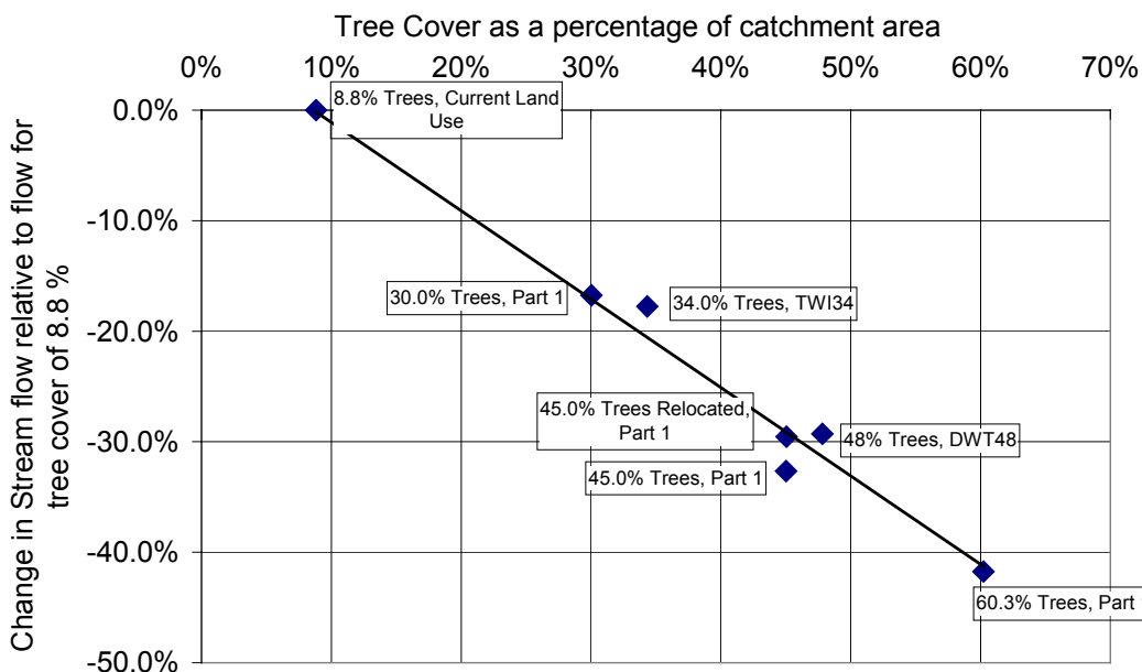
■ Figure 5-2 Hamilton/Dry case study area: change in modelled stream flow versus tree cover. The line shown is the linear regression line that passes through the point representing current conditions (i.e. stream flow = 149 mm/year).
