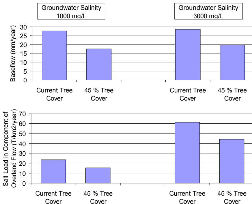
■ Figure 4-11 Hamilton/Dry Creek: Comparison of the effects of groundwater salinity on different components of salt and water balance.
