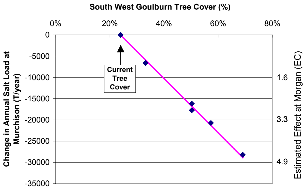
■ Figure 5-7 Change in modelled Salt Load at Murchison vs tree cover in the South West Goulburn. An estimate of the effect on EC at Morgan is given on the axis on the right.
