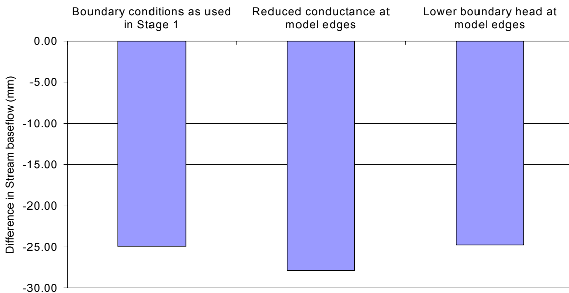
■ Figure 4-8 Difference in stream baseflow between current land use and 45 % tree cover for three applications of the GHB boundary condition. (See also Figure 4-7)
