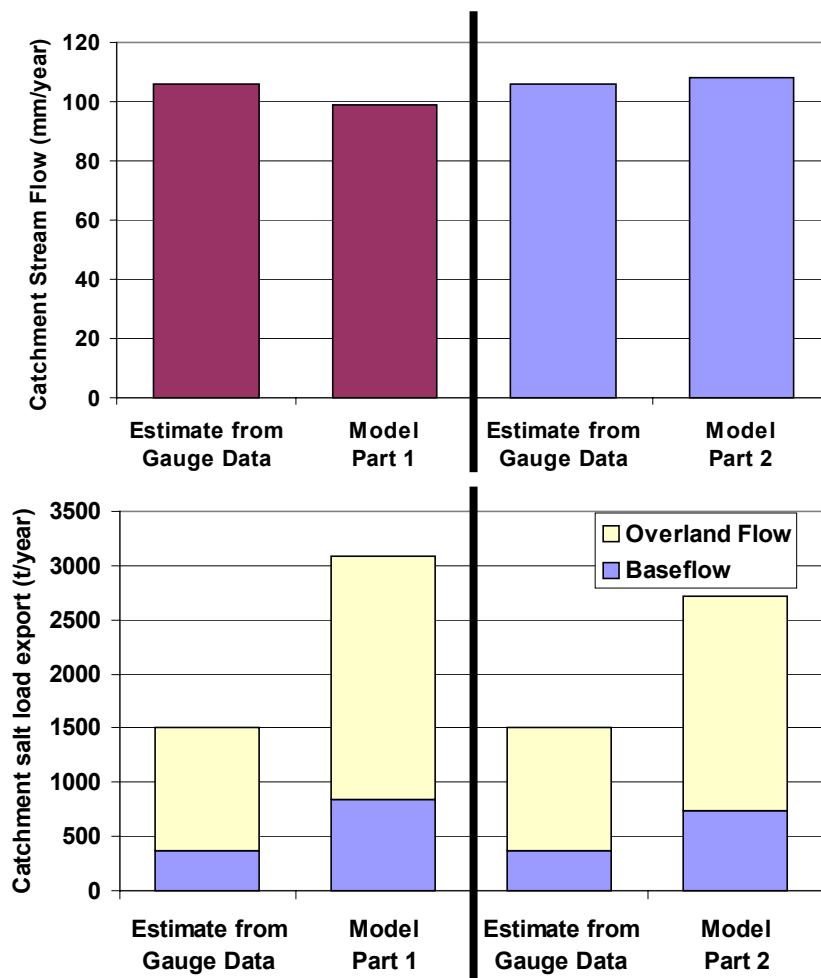
■ Figure 4-13 Gardiner Creek: comparison of stream flow and salt load as modelled in Part 1 and Part 2 of the project. Model results are also compared with estimates from the stream gauge network.
