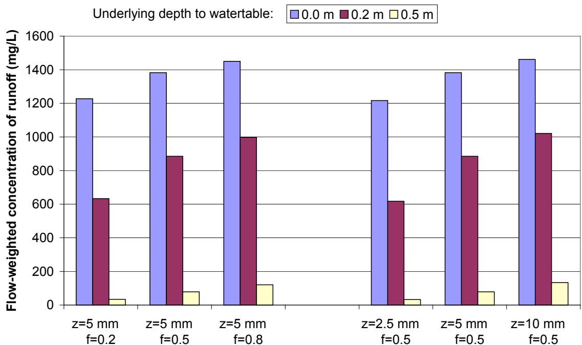
■ Figure 4-1 Flow weighted concentration of runoff (mg/L) for three underlying depths to watertable. The effect of a variable f_{\text{salt}} is shown on the left of the figure and the effect of a variable z_{\text{salt}} is shown on the right.
