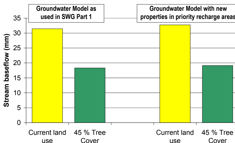
■ Figure 4-5 Gardiner Creek case study area: comparison of the stream baseflow component before and after adoption of the new representation of aquifer properties around the Moormbool fault.
