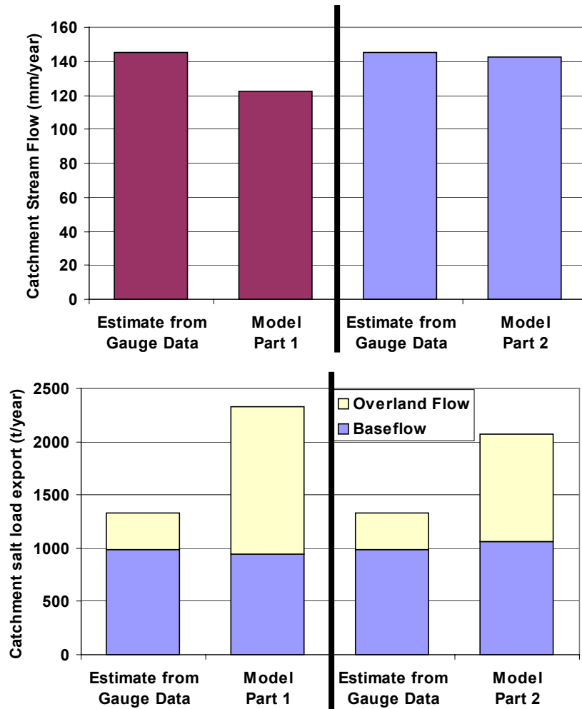
■ Figure 4-14 Hamilton/Dry Creek: comparison of stream flow and salt load as modelled in Part 1 and Part 2 of the project. Model results are also compared with estimates from the stream gauge network.
