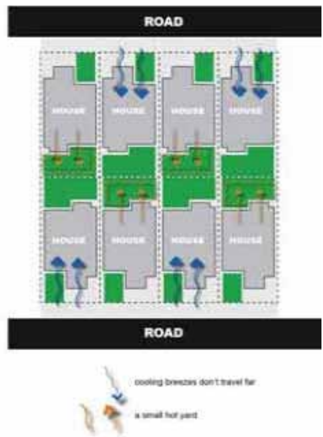
Figure 2. A wide plan form on a narrow lot restricts circulation of cooling breezes.
