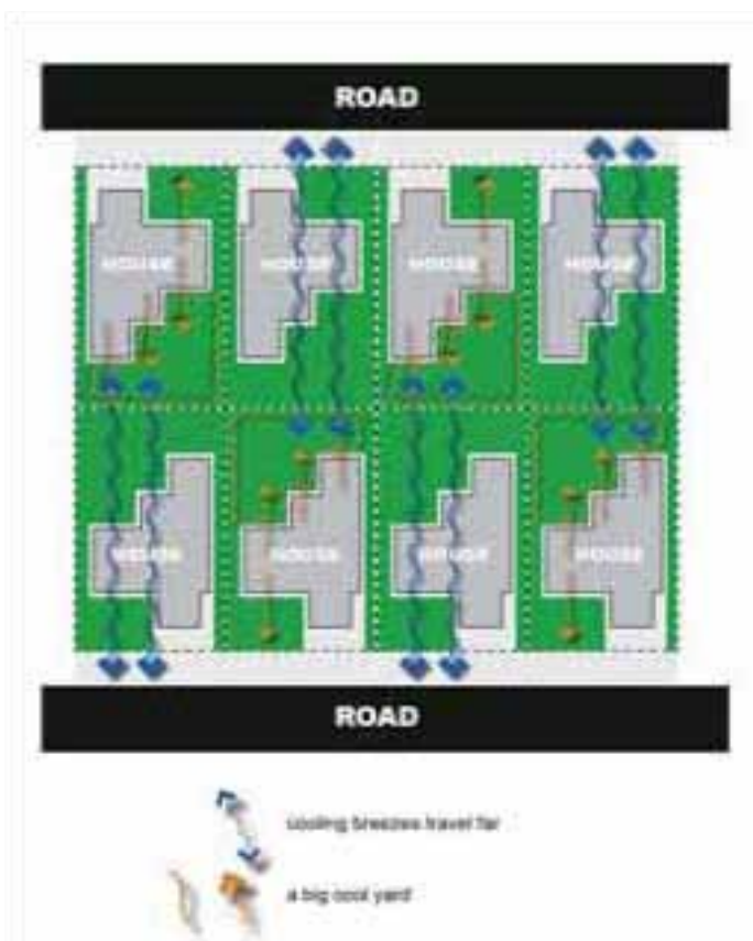
Figure 1. A thin plan form on a wide lot allows maximum circulation of cooling breezes.
