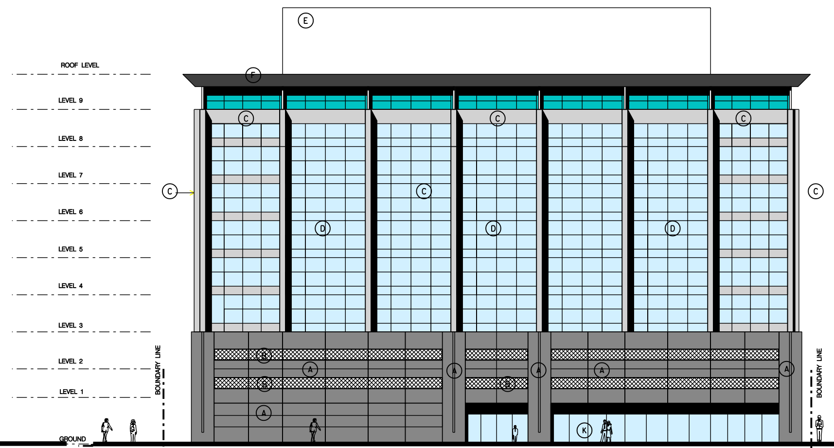
Eastern Elevation
