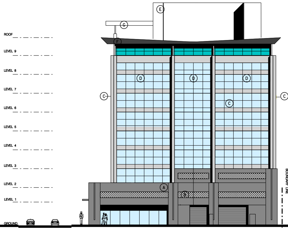
Southern Elevation
