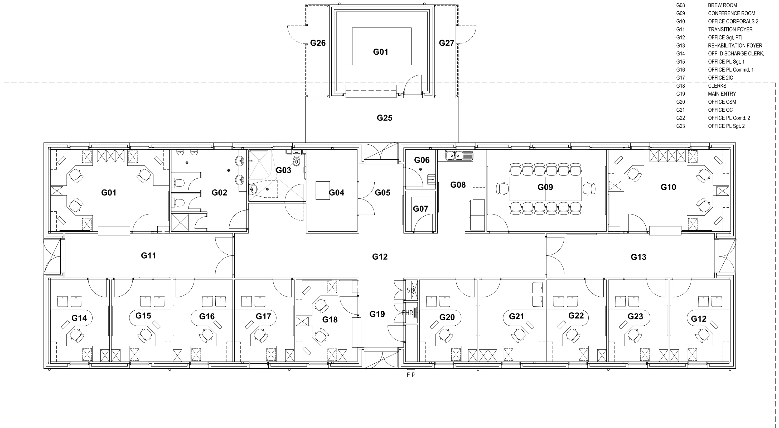
Attachment 84 Transition Rehabilitation Headquarters Building Floor Plan
