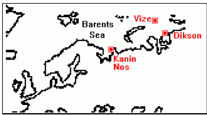
Kanin Nos, Dikson, & Vize, Arctic Russia Annual Mean Temperature 1916-1999
