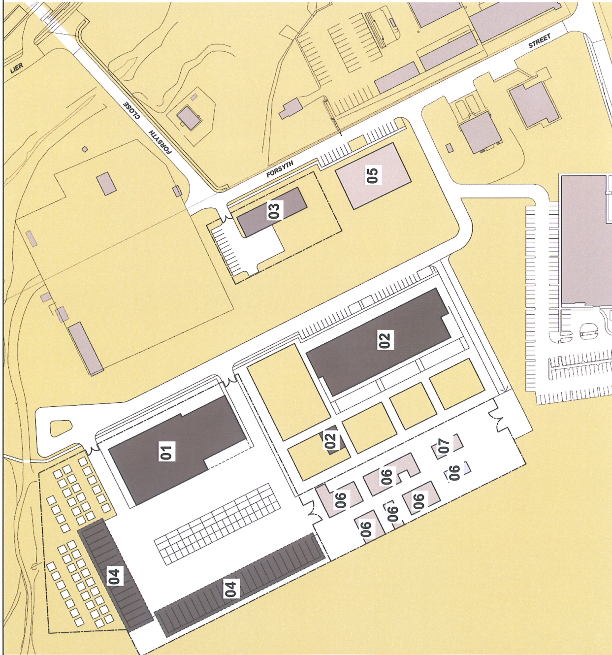
Attachment 14: Site Plan New Enoggera Close Training Area, Mission Rehearsal Exercise, Battle Simulation Centre & Explosive Hazards Centre Precinct
