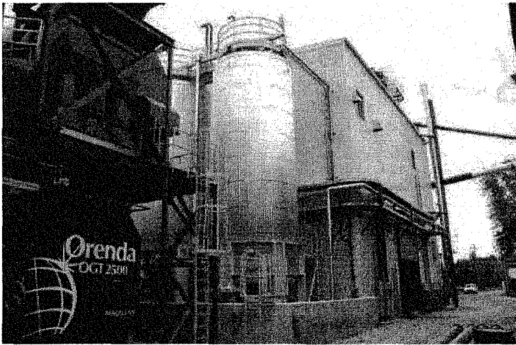
Figure 9: Dynamotive Plant in Canada (source: Dynamotive)
