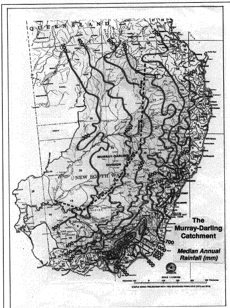
Figure 12. Rainfall Isohyets (mm)
