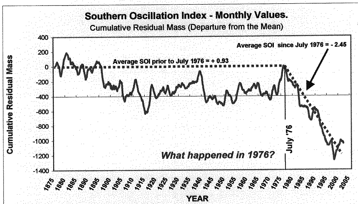
Figure 3. Trends in the Southern Oscillation Index
