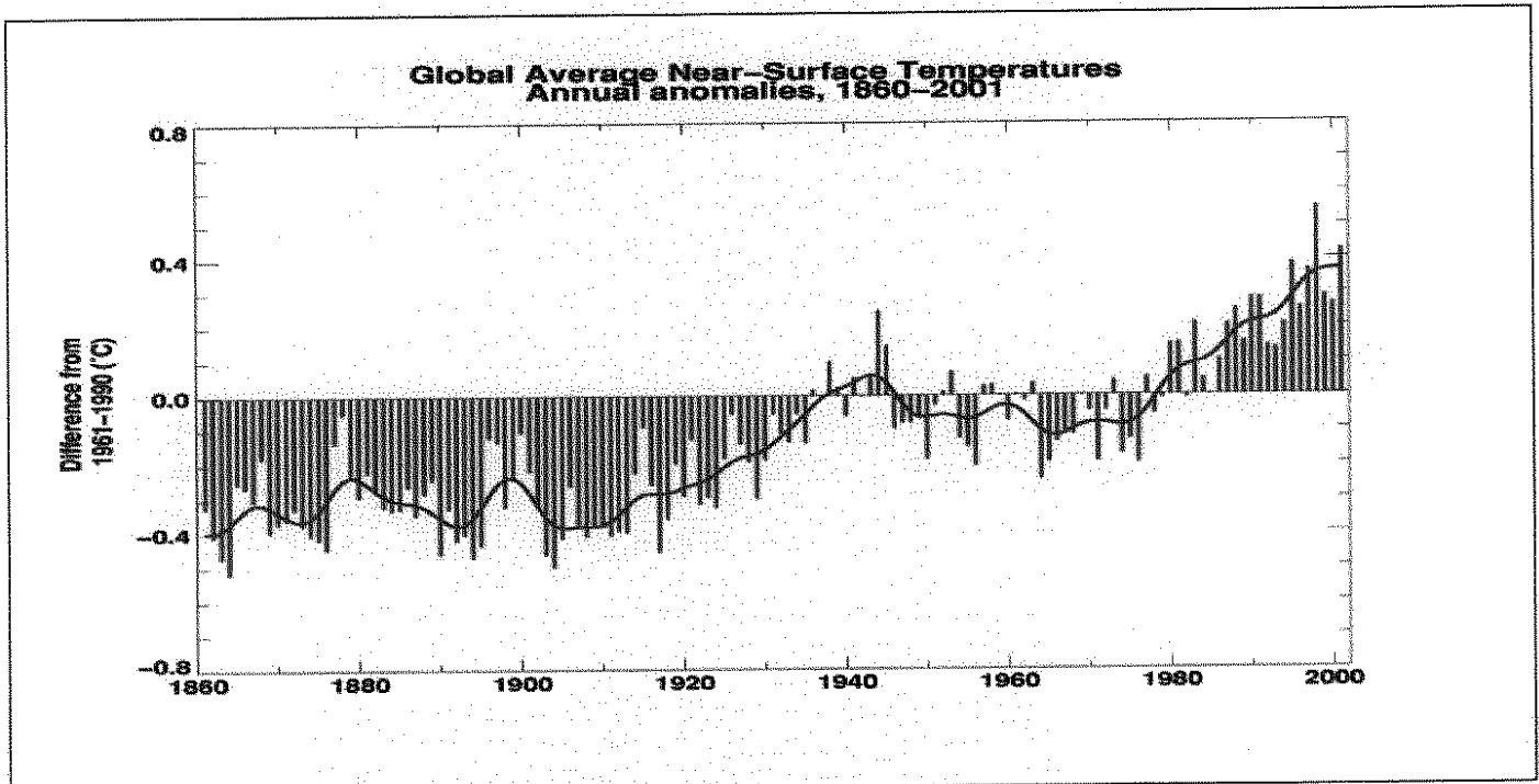
Figure 4. Change in Global Temperatures.
