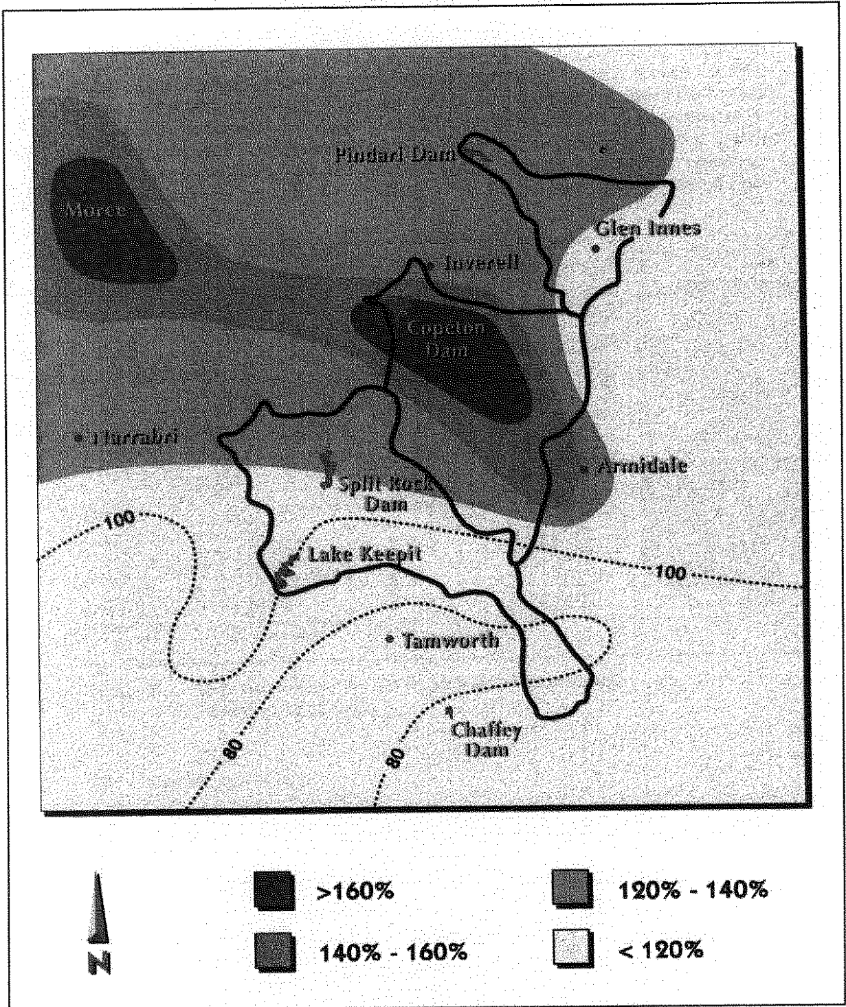
Figure 9. Rainfall Distribution 18 Nov 1994 – 12 Feb 1995 (Percent of Normal)
