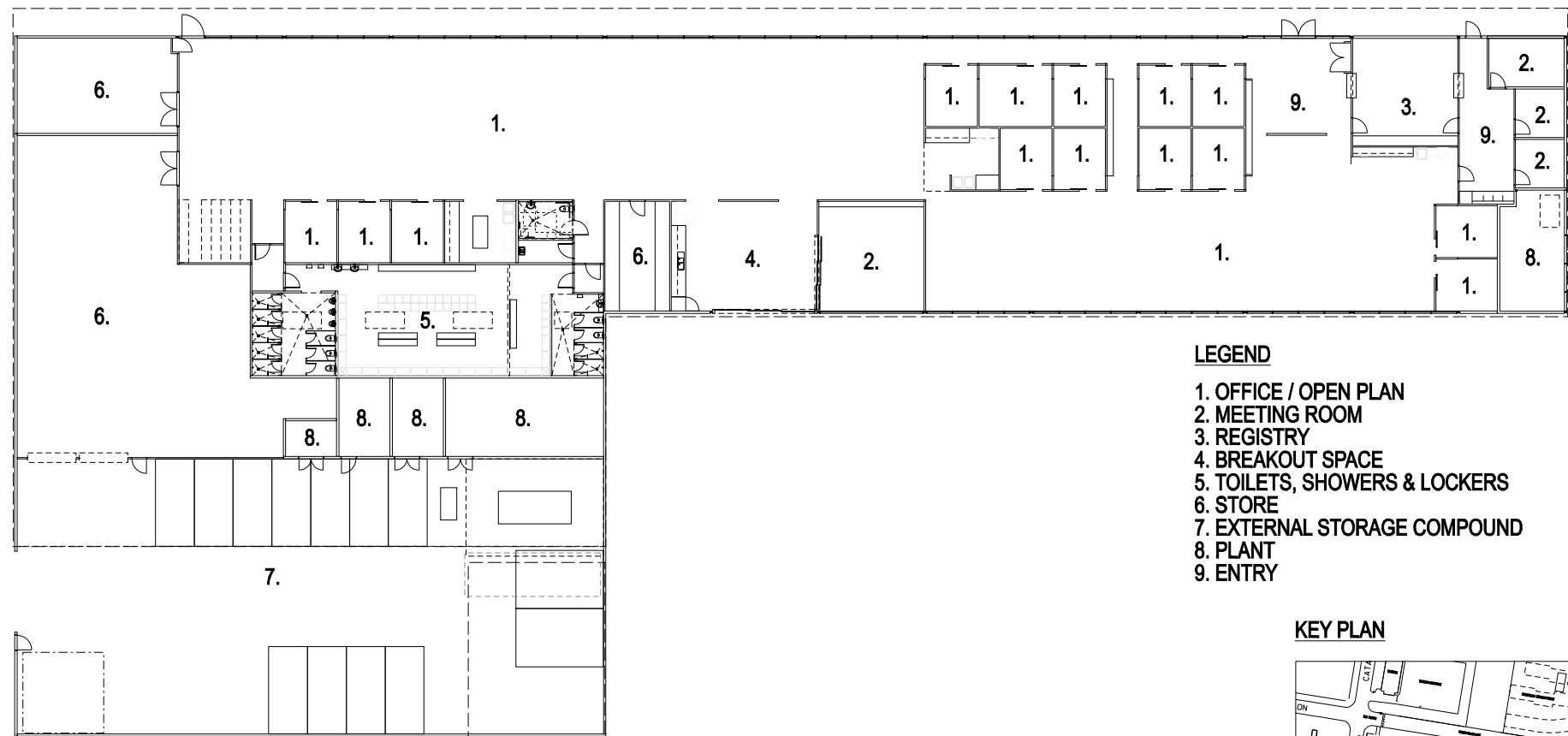
GROUND FLOOR
