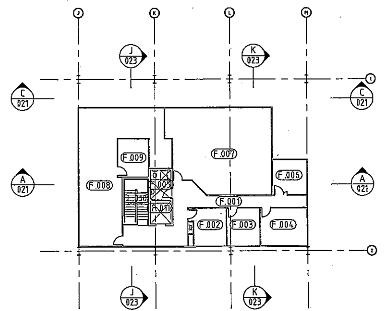
FIRST FLOOR PLAN SCALE 1:200
