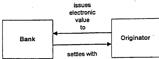
FIGURE 4.6 Originator
