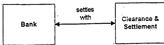
FIGURE 4.7 Clearance & Settlement
