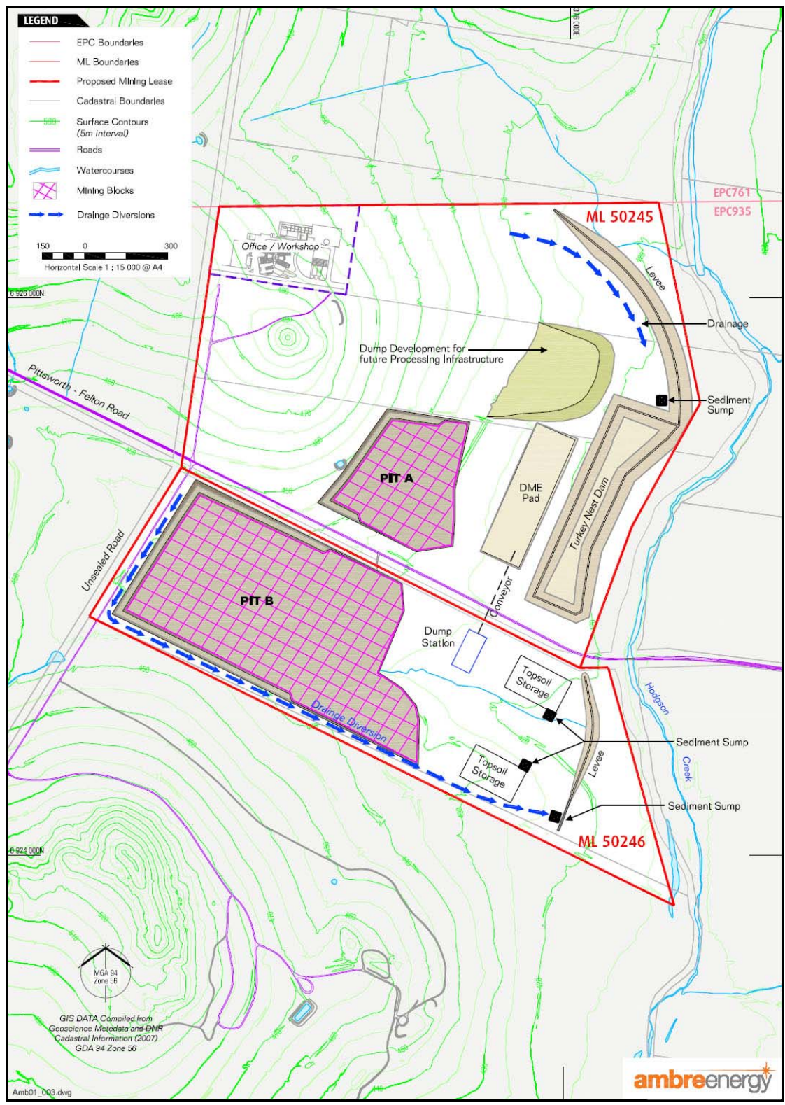
Figure 4, Demonstration Stage Mine and Infrastructure layout plan
