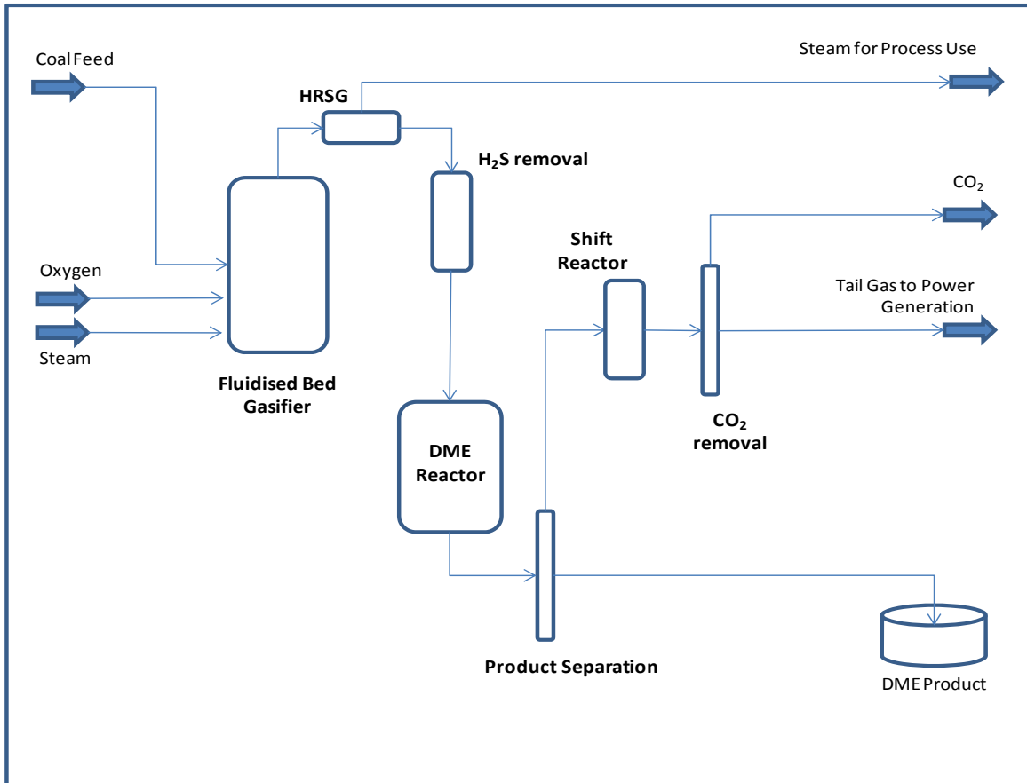
Figure 5, Pilot Plant Flow Diagram
