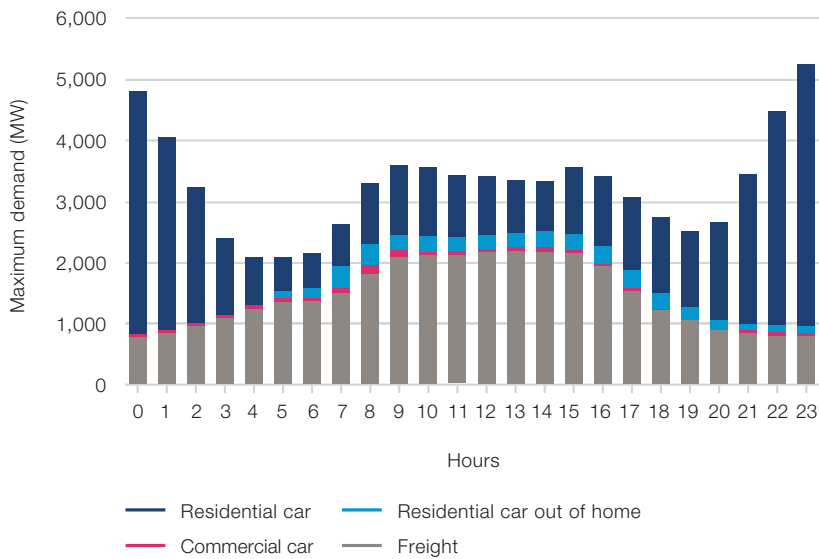
Figure 27: Load profile – incentivised
