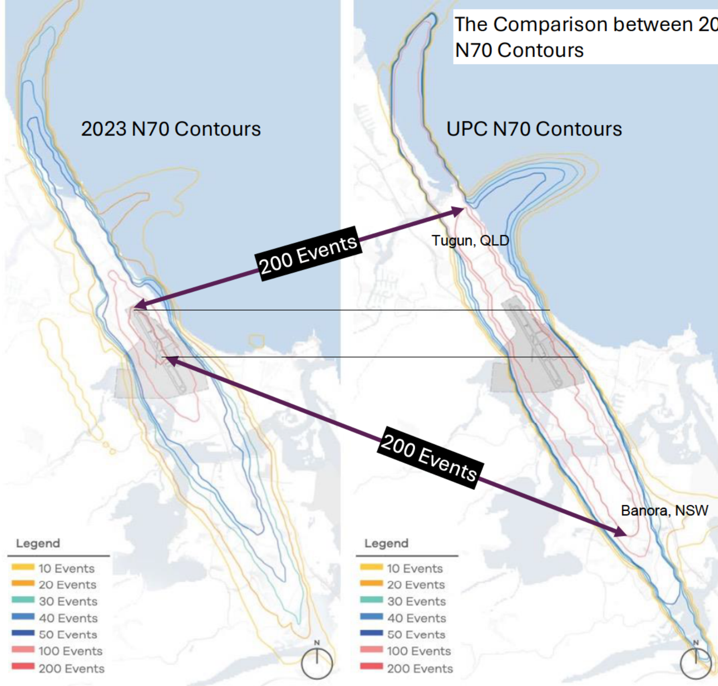
Figure 7.2.11 – 2023 N70 Contours
