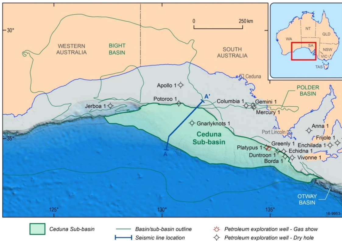
Figure 3: Ceduna Sub-basin.
