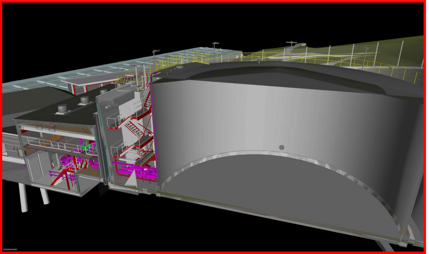
SECTION THROUGH KNOLL TANK & FUEL PUMP HOUSE
