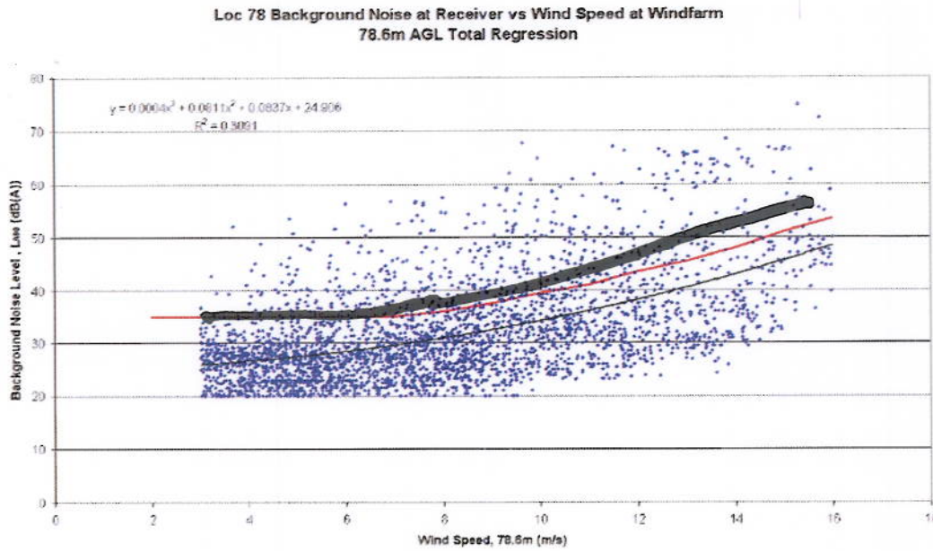
Figure 12.5 – Background noise at receiver Residence 78 versus wind speed at wind farm
