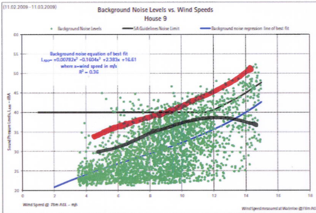
Figure 4: House 9 background noise monitoring results and noise limits
