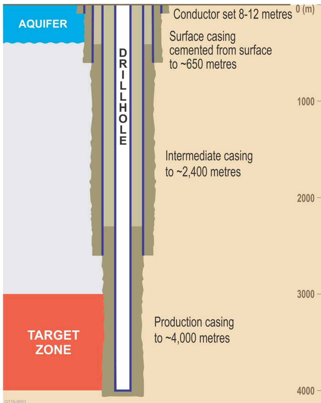
Figure 6: Indicative well design. Wells are designed to meet engineering and regulatory requirements for specific well objectives. Casing size, weight, grade, depths and cement volumes will be varied to meet engineering design specifications.
