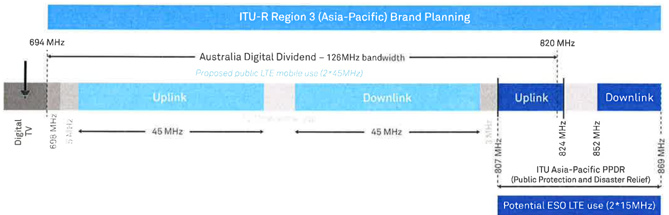
Figure 1: 800 MHz PPDR Frequency Plans
