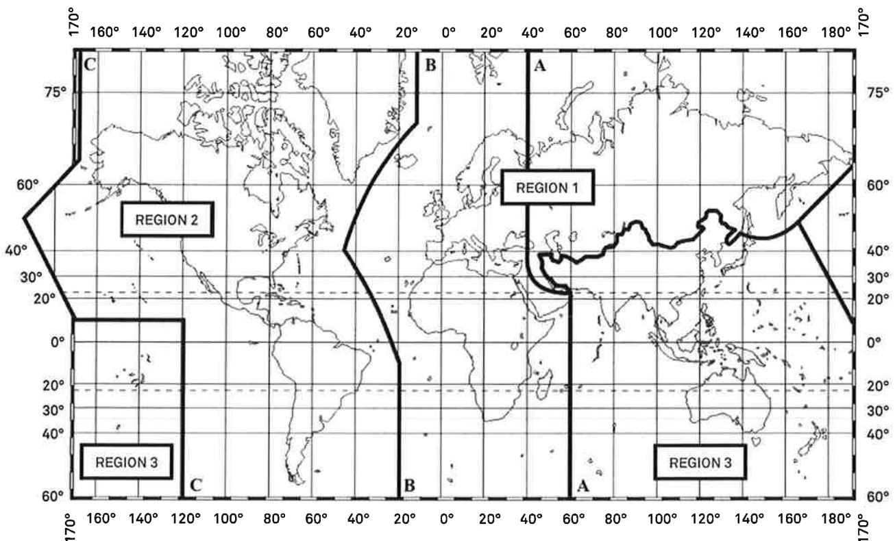
Figure 2: ITU Regions
