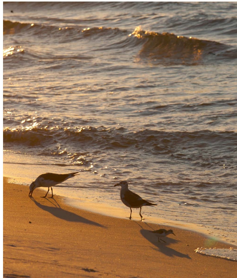
Some early restoration projects are supporting bird habitats.
