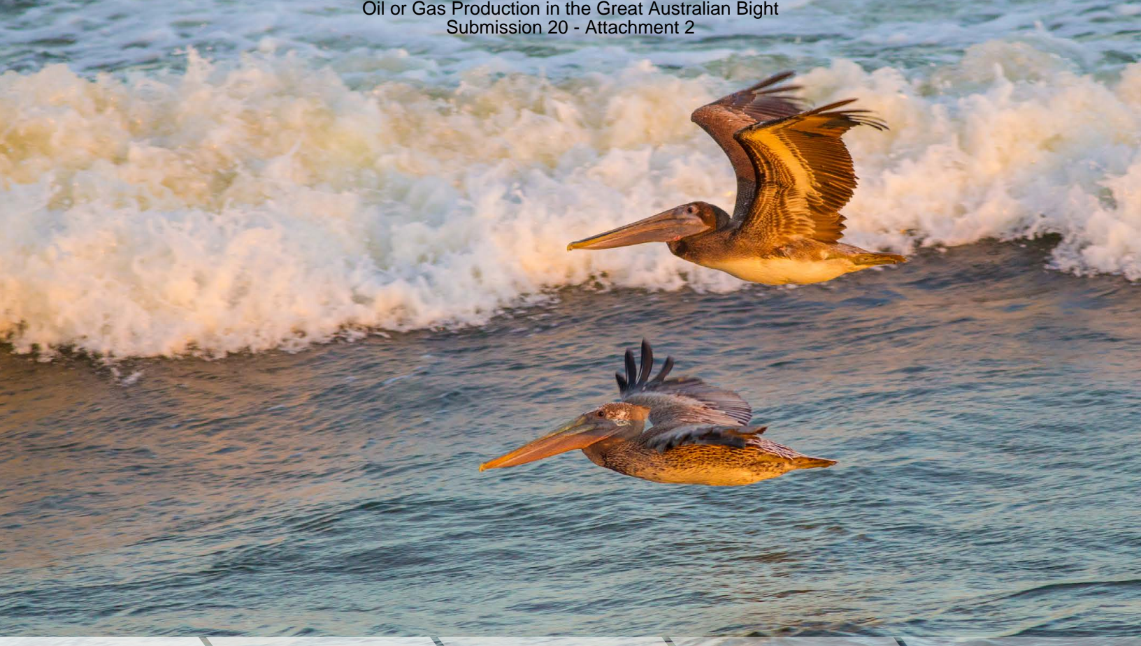
Brown pelicans travel along a Gulf shoreline, September 2014.
