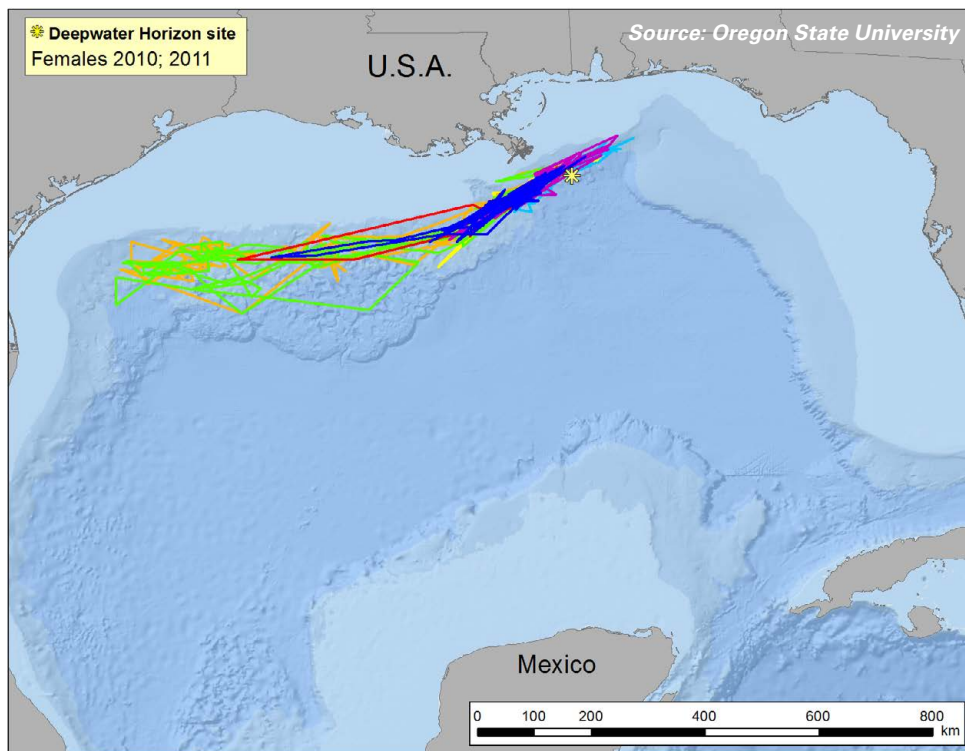
Satellite telemetry tracks sperm whales in the northern Gulf.
