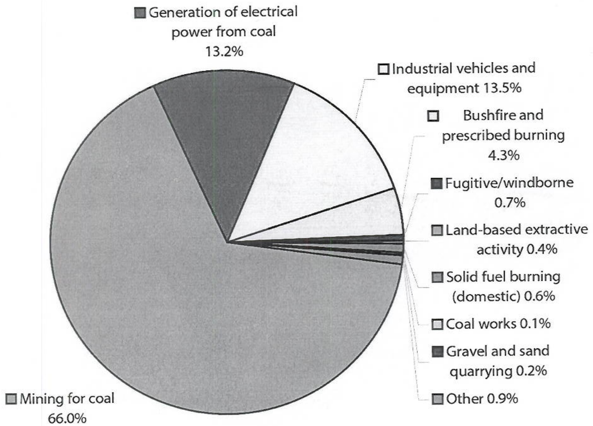
Figure 5: PM 2.5 emissions from all sectors in the Upper Hunter Region – 2008 Air Emissions Inventory
