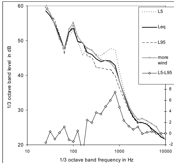
Figure V.5: 1/3 octave band levels at façade of dwelling P during beating ( L_{eq} , L_5 and L_{95} ) and when wind speed is picking up ( L_{eq} ); lower line: dynamic range ( R_{f,90} ) of 1/3 octave band
