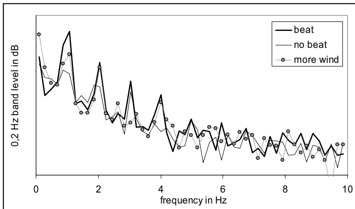
Figure V.6: sound power spectrum of A-weighted broadband immission sound level at façade of dwelling P when beating is distinctly or not audible and with slightly increased wind speed. The ordinate spans 20 dB.
