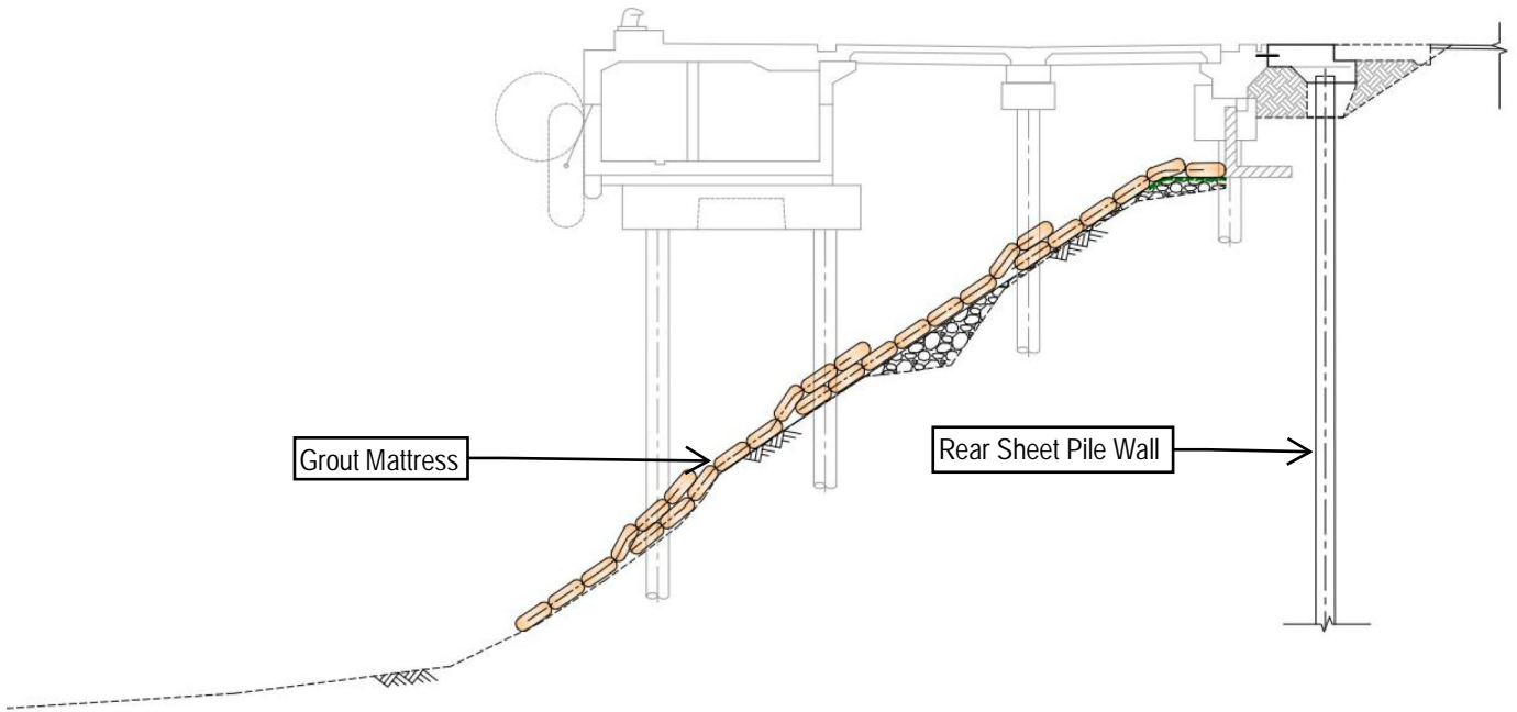
SECTION 1: Grout Mattress and Rear Sheet Pile Wall Fleet Base East 2-5
