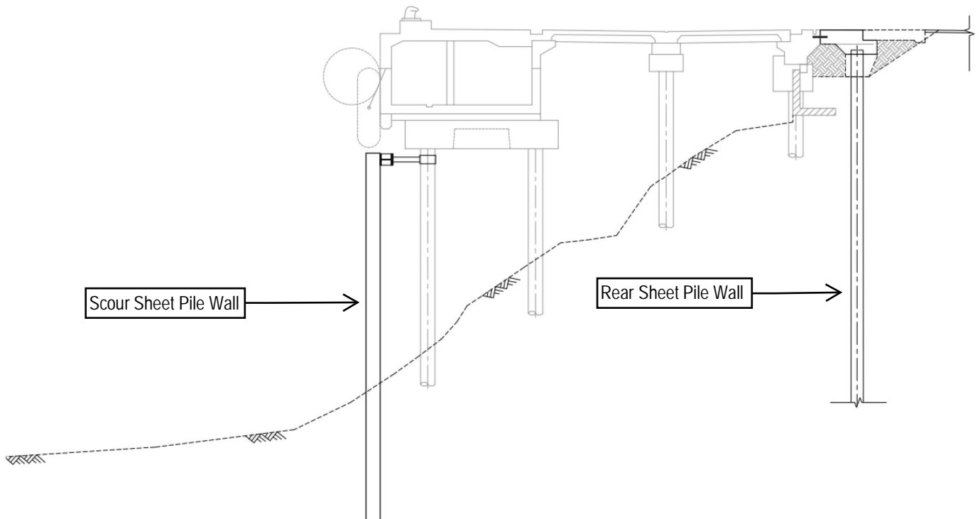
SECTION 2: Scour Sheet Pile Wall and Rear Sheet Pile Wall Fleet Base East 3
