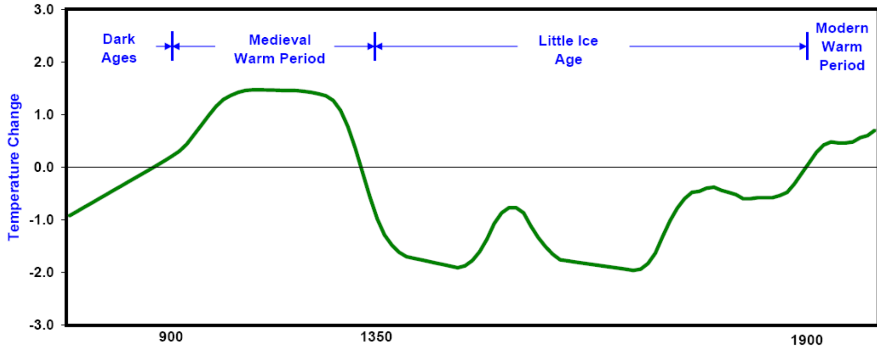
Figure 6: Medieval Warm Period – Little Ice Age
