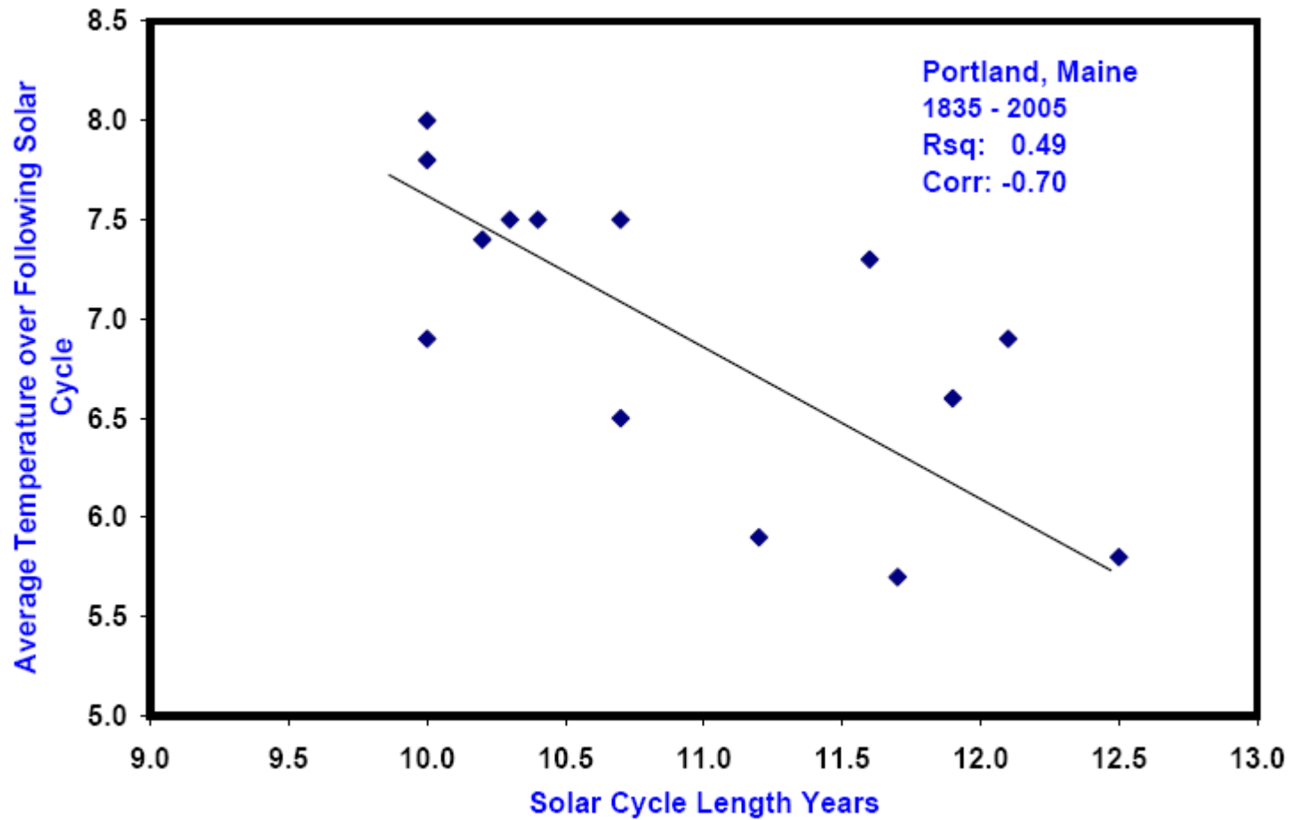
Figure 13: Portland, Maine – Solar Cycle Length Relative to Temperature
