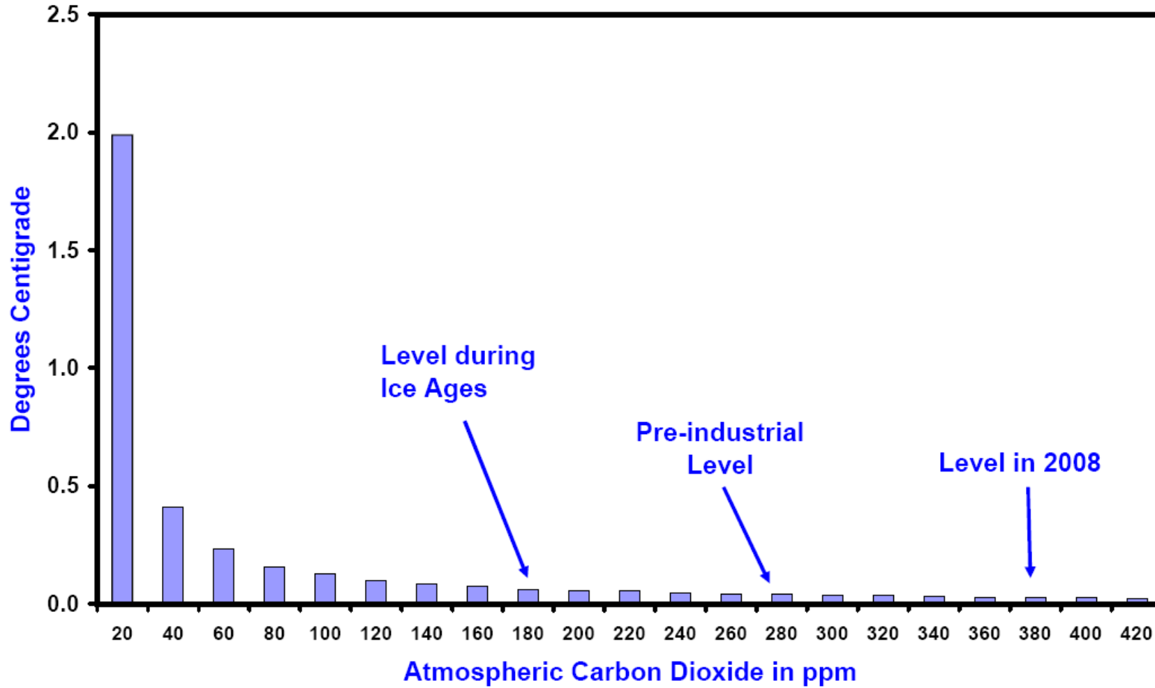
Figure 30: The Warming Effect of Carbon Dioxide
