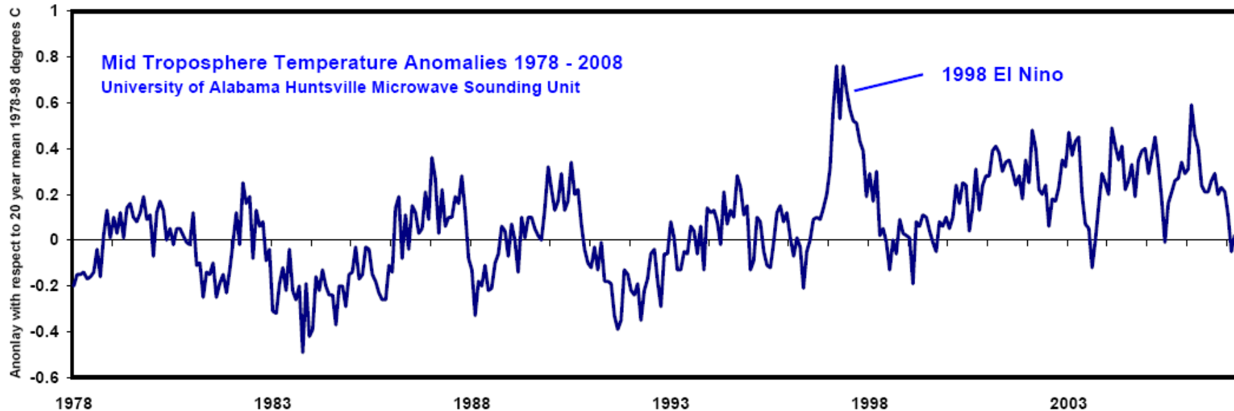
Figure 1: The Satellite Record
