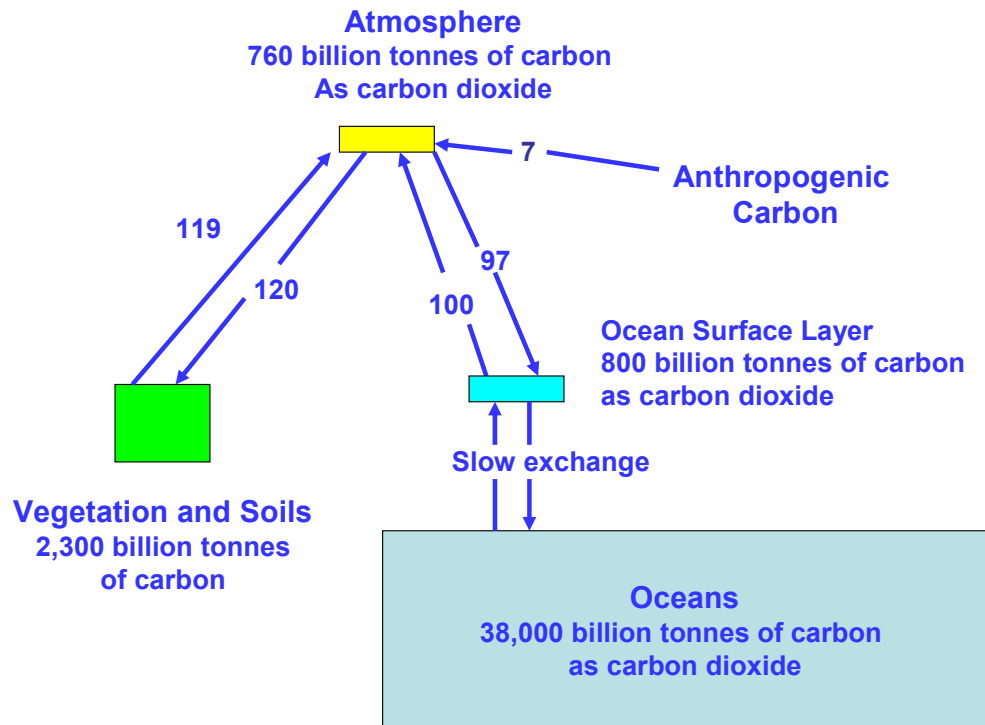
Figure 37: Annual Carbon Flux between the Oceans, Vegetation and Soils, and the Atmosphere
