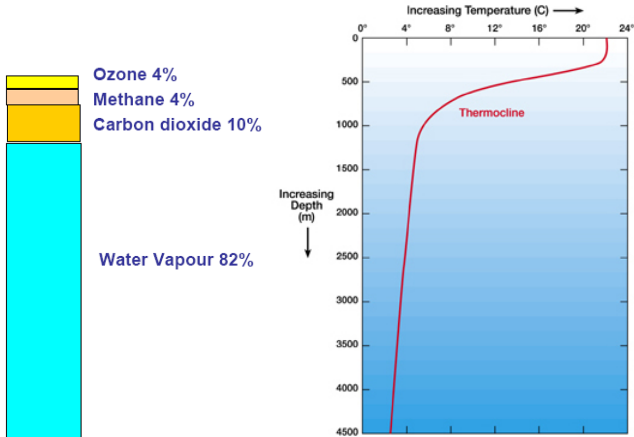
Figure 35: Relative Contribution of the Major Greenhouse Gasses
