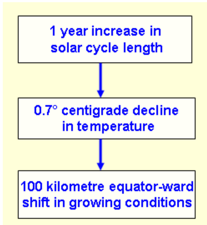
Figure 25: The Consequential Climate Shift
