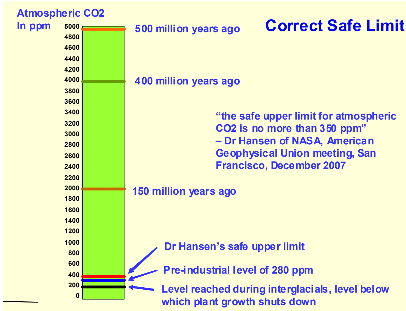
Figure 32: Correct Safe Limit
