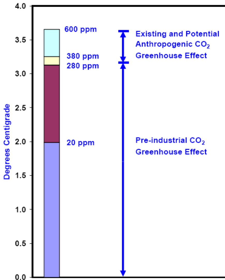
Figure 31: Relative Contributions of Pre-industrial and Anthropogenic CO 2
