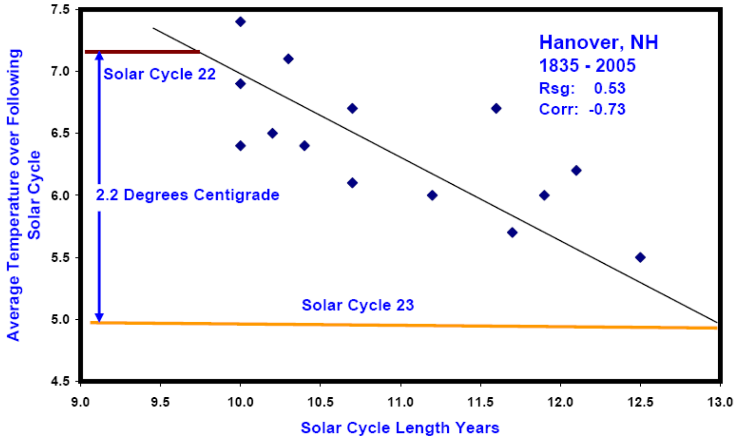
Figure 14: Hanover, New Hampshire with Solar Cycle 22 Plotted Relative to Solar Cycle 23
