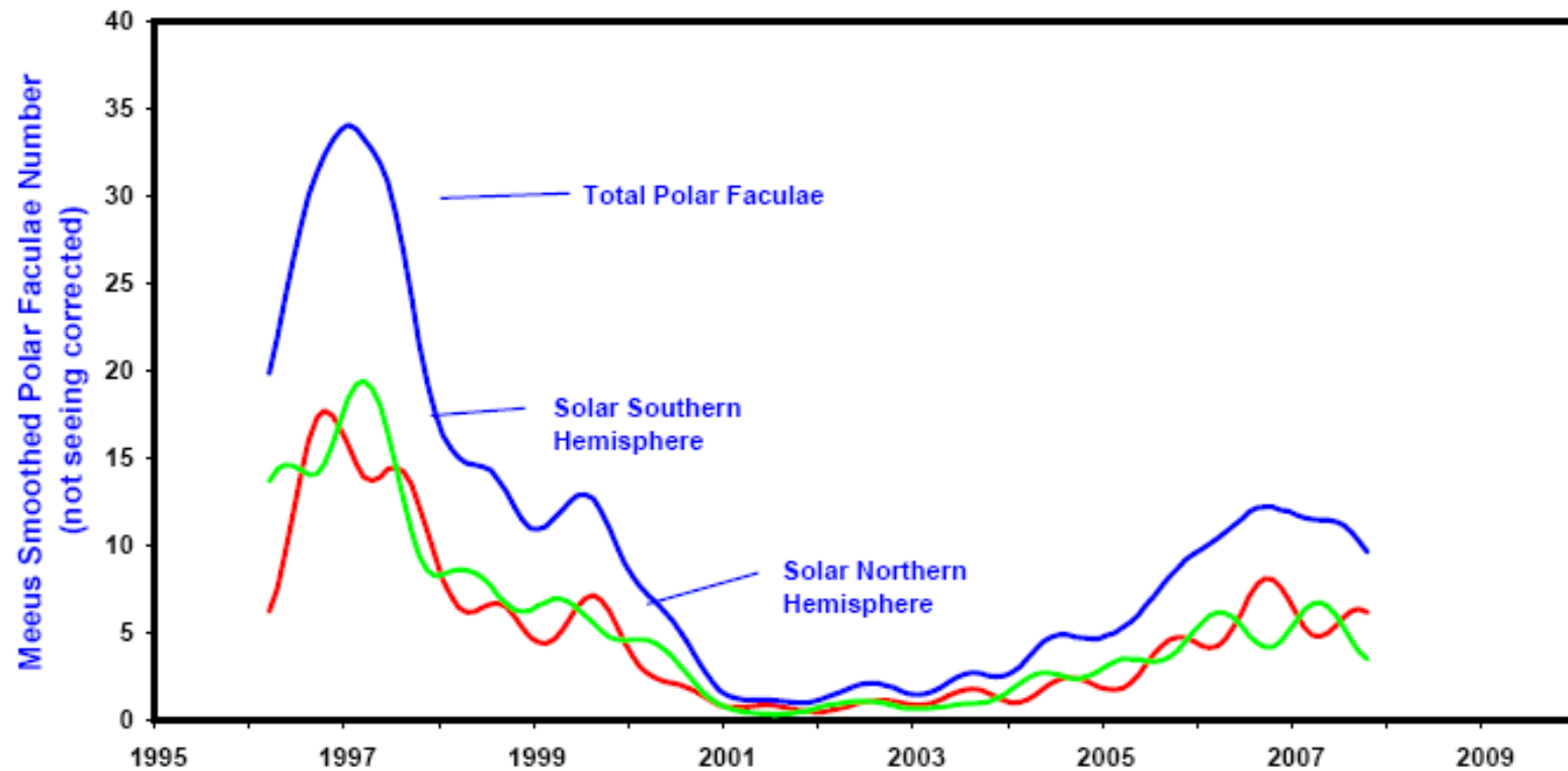
Figure 21: Polar Faculae on the Sun
