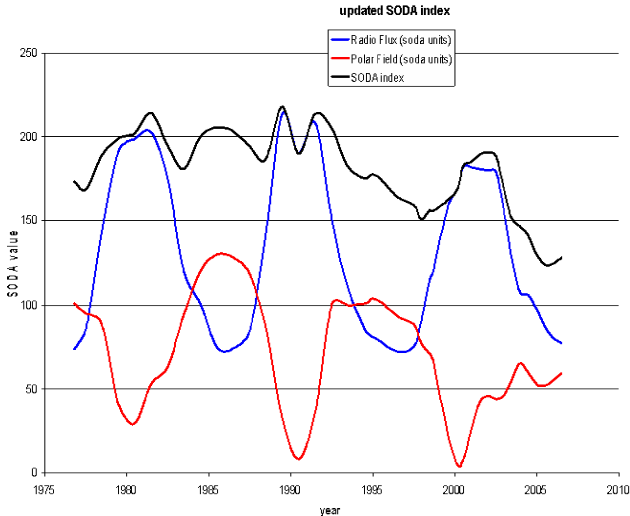
Figure 20: The Solar Dynamo Index
