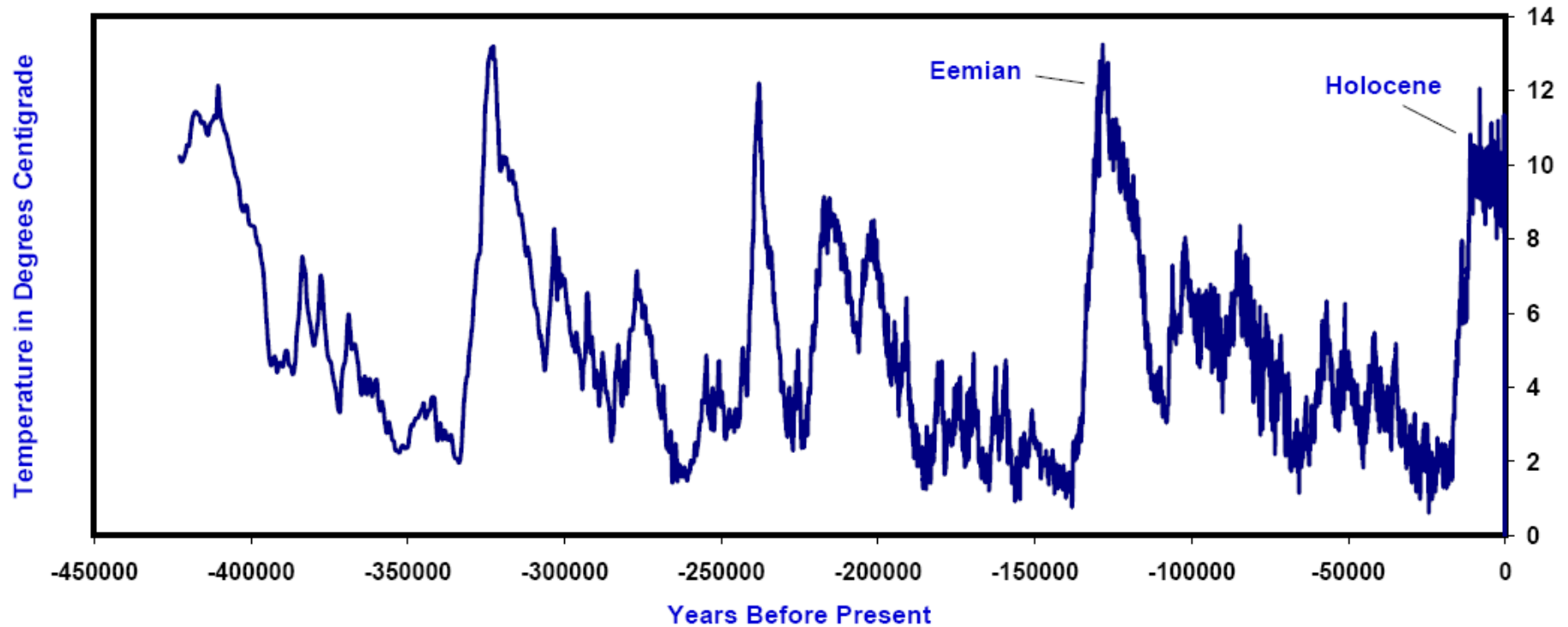
Figure 8: Vostok Ice Core Temperature Profile
