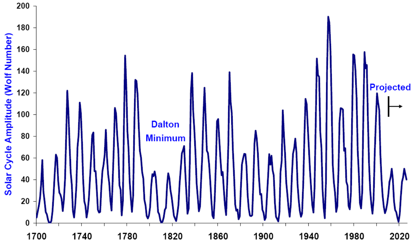
Figure 10: Solar Cycles from 1700 and Projected to 2030
