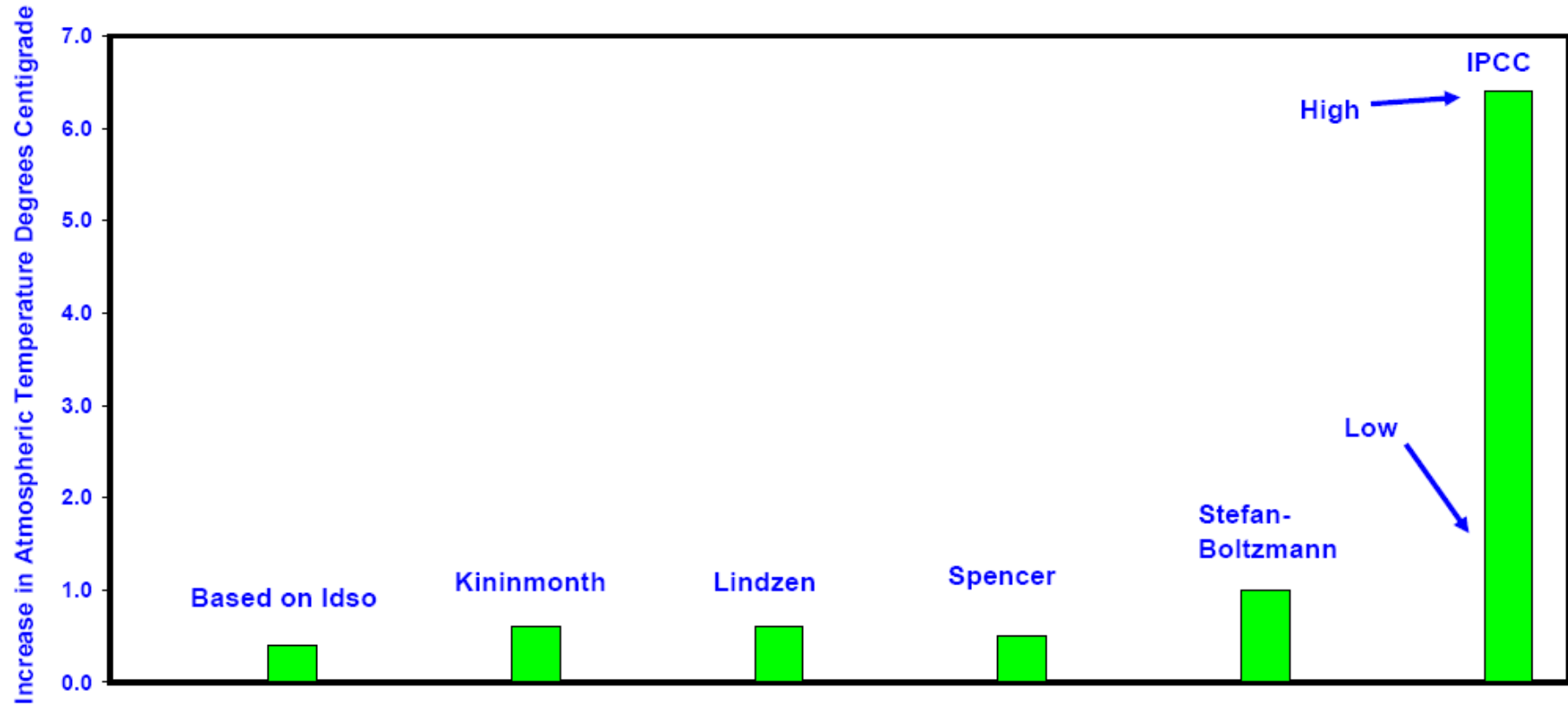
Figure 33: Comparison of Climate Sensitivity Estimates
