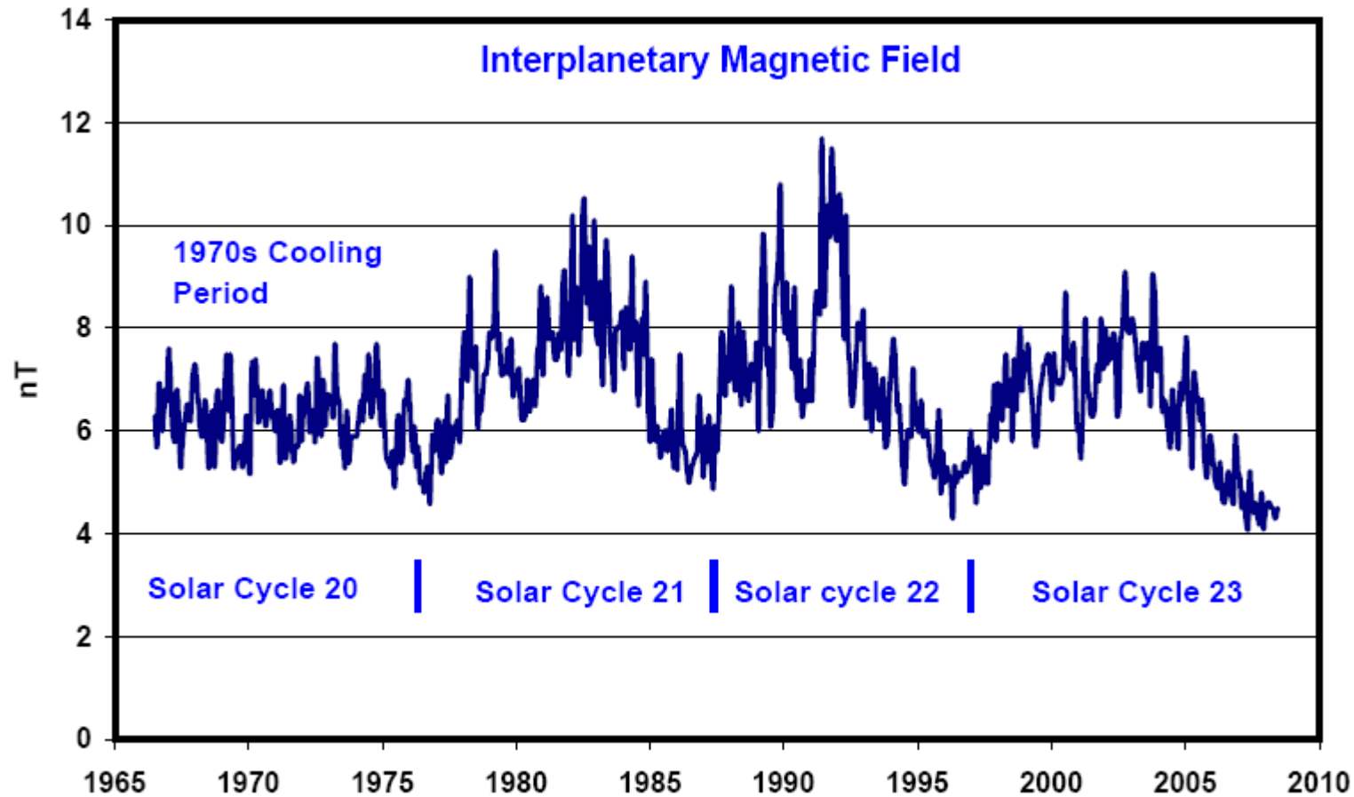
Figure 22: Interplanetary Magnetic Field
