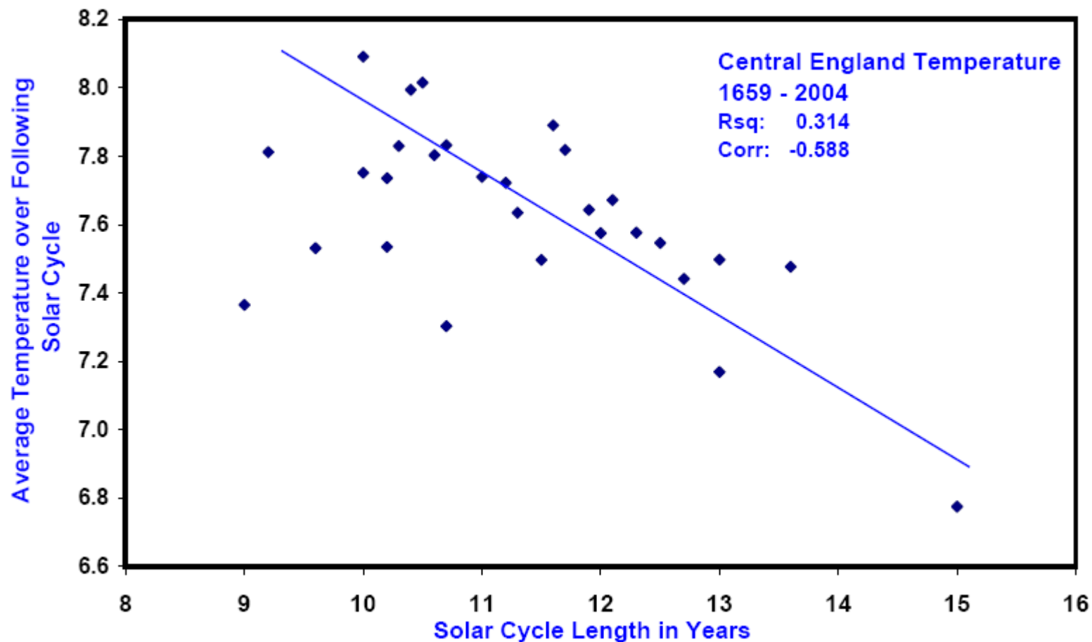
Figure 12: Solar Cycle Length Relative to Temperature
