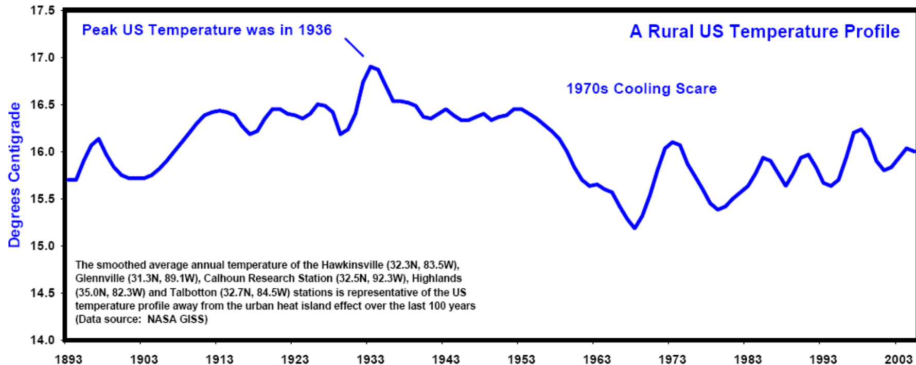
Figure 4: A Rural US Temperature Profile
