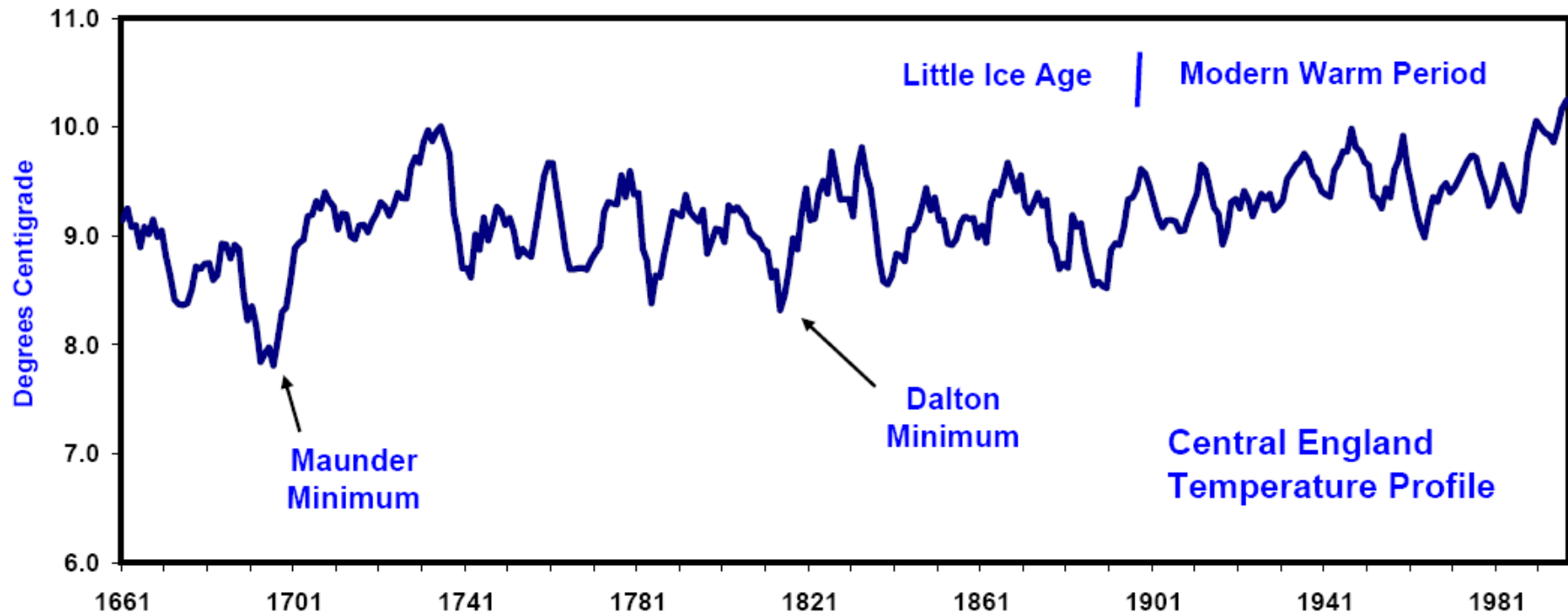
Figure 5: A 300 Year Thermometer Record
