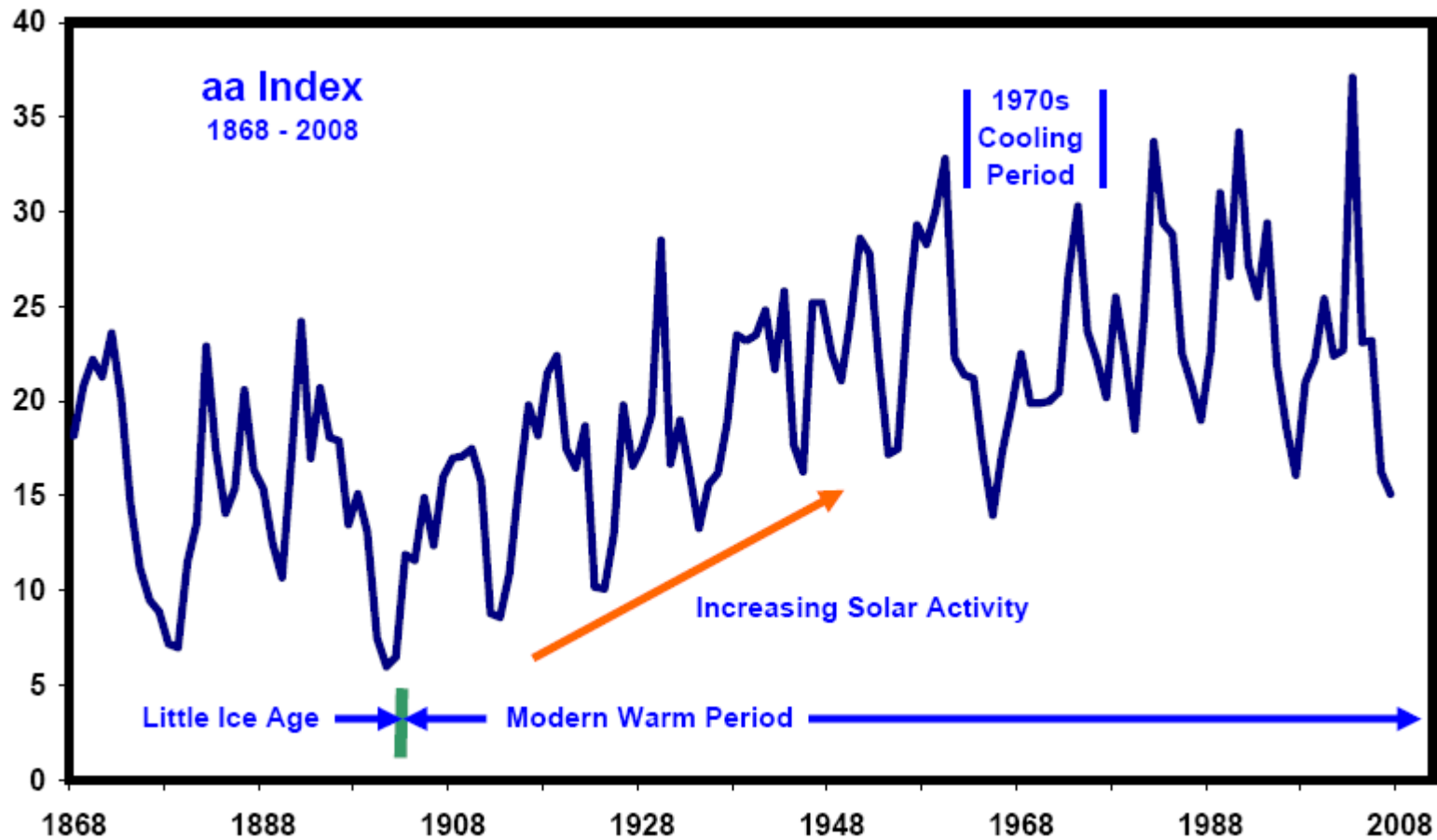
Figure 28: The aa Index from 1868 to 2008
