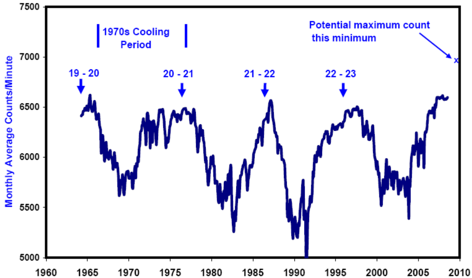
Figure 23: Oulu, Finland Neutron Monitor Count 1960 – 2010
