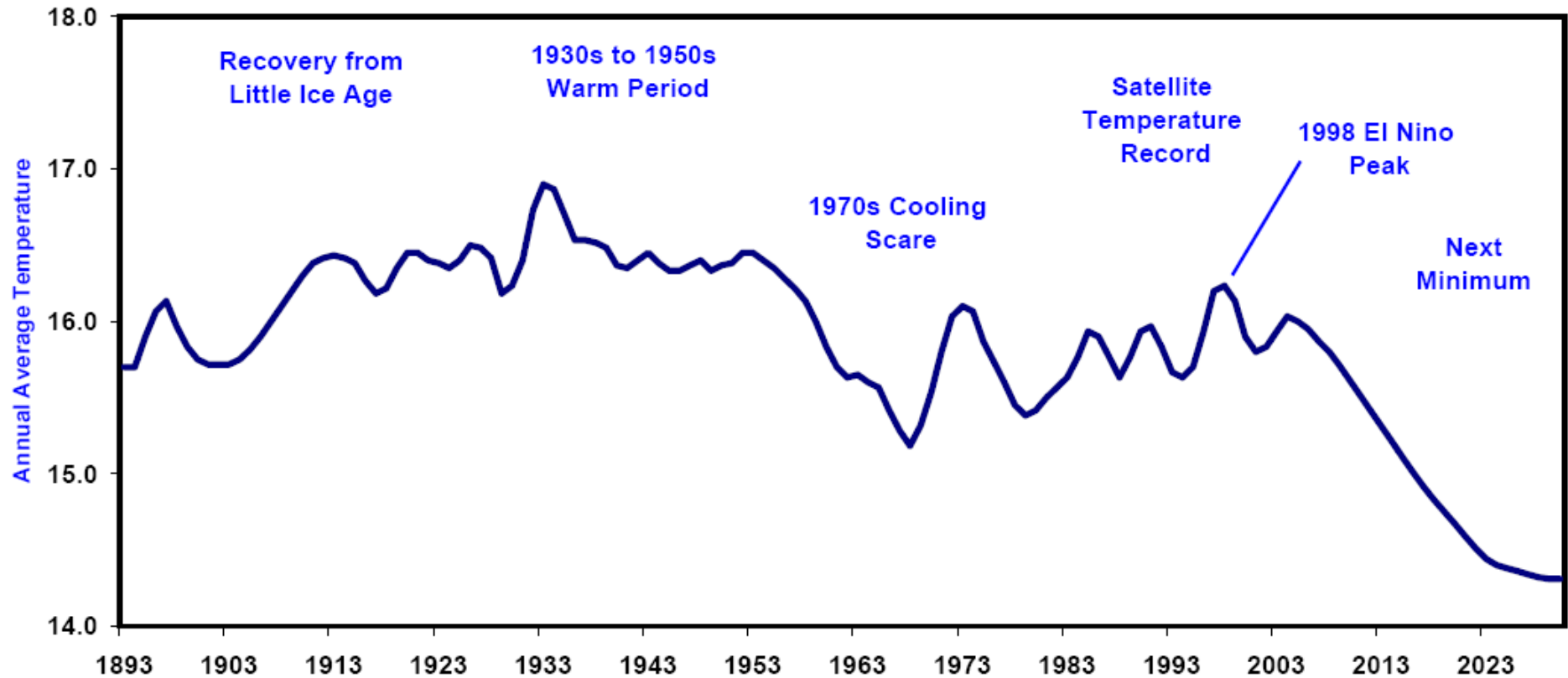
Figure 24: Projected Mid-latitude US Temperature Profile to 2030
