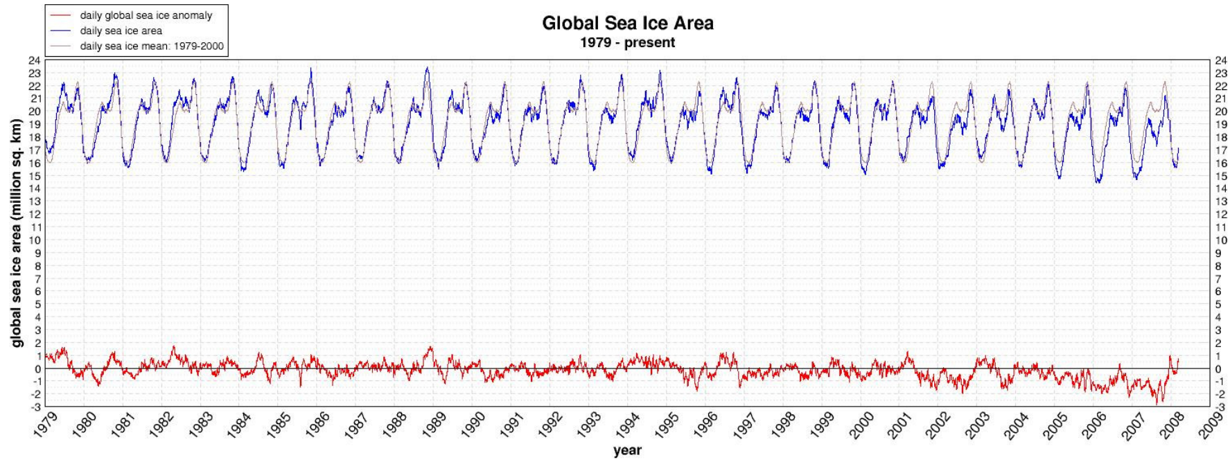
Figure 2: Global Sea Ice Area
