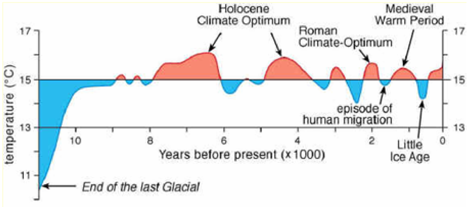
Figure 7: The Holocene Optimum
