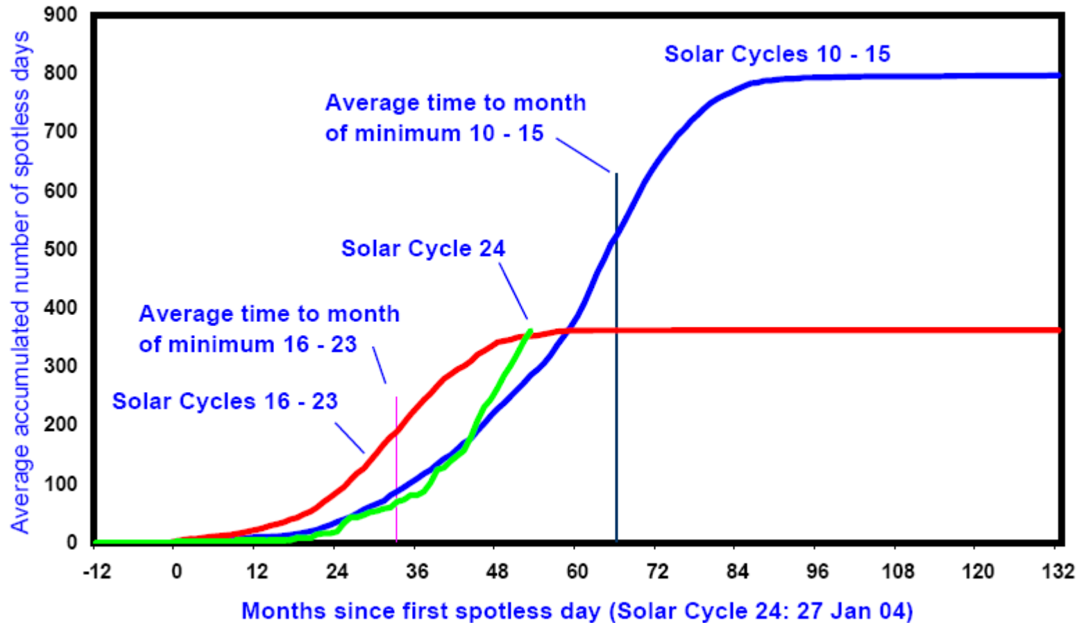
Figure 15: Accumulated Number of Spotless Days – Solar Cycles 10 to 15 compared to Solar Cycles 16 to 23
