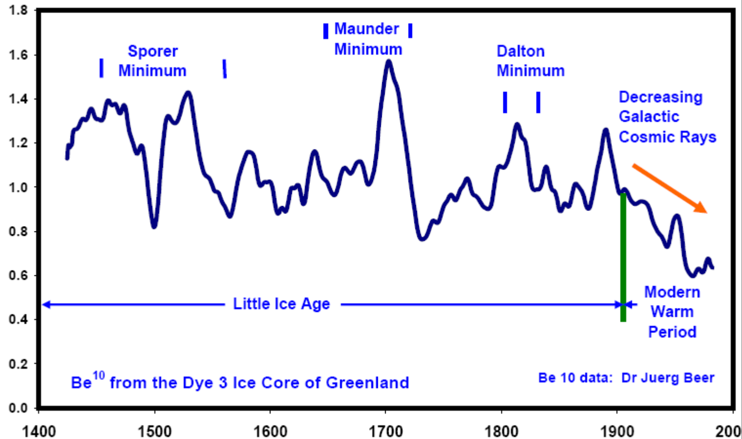
Figure 27: Be^{10} from the Dye 3 Ice Core of Greenland
