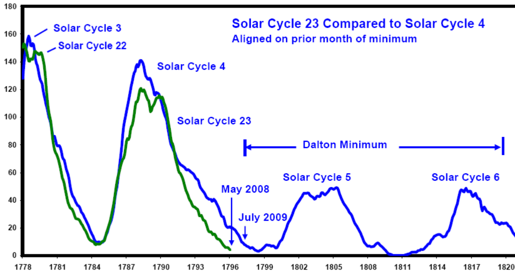
Figure 18: A Repeat of the Dalton Minimum?
