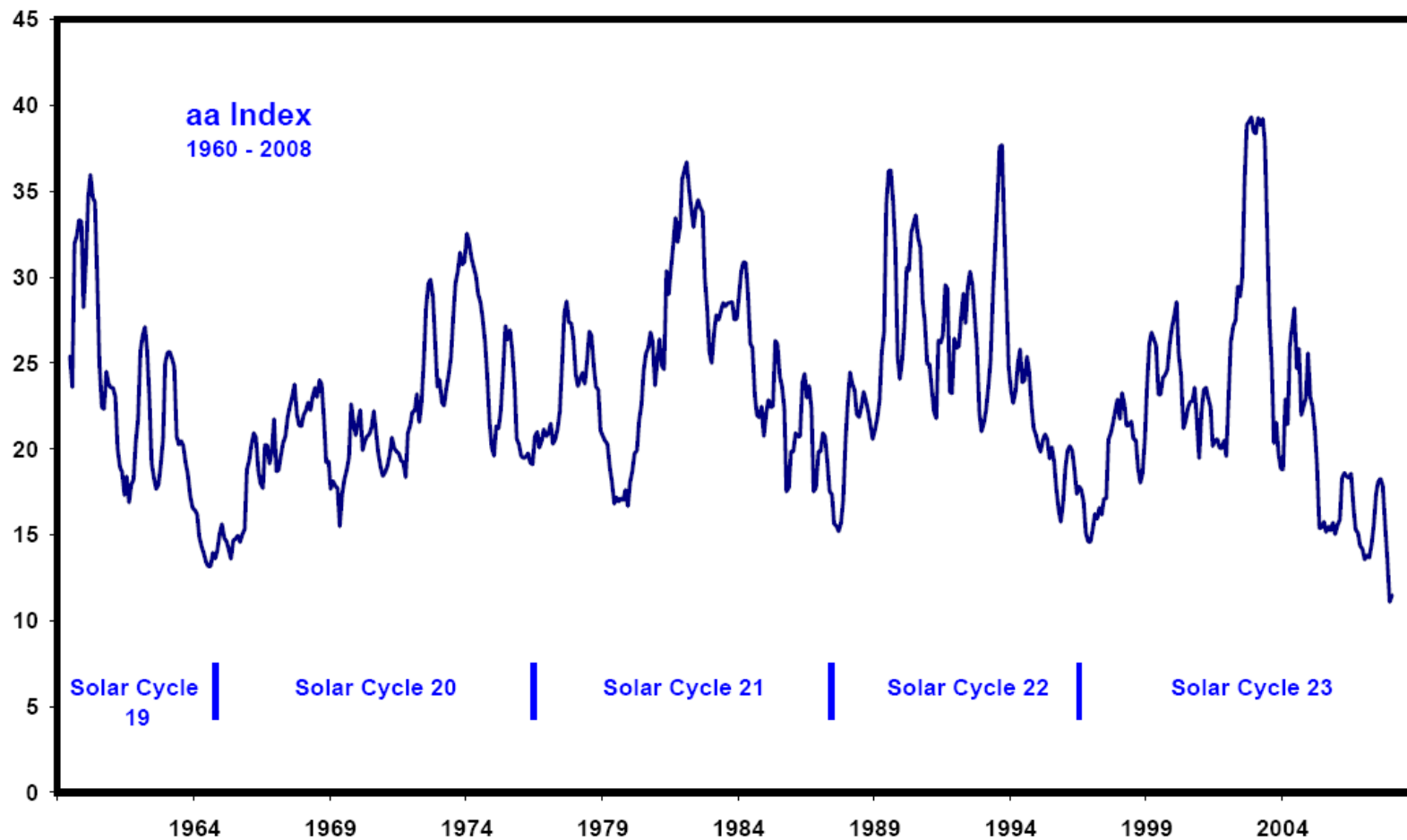
Figure 29: The aa Index 1960 – 2008
